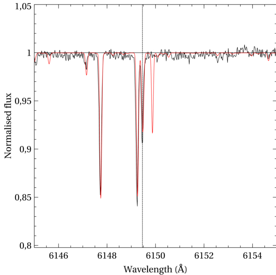
Figure 1. from Richard Monier 2026 Res. Notes AAS 10 doi:10.3847/2515-5172/aea570 https://dx.doi.org/10.3847/2515-5172/aea570 © 2026. The Author(s). Published by the American Astronomical Society.
