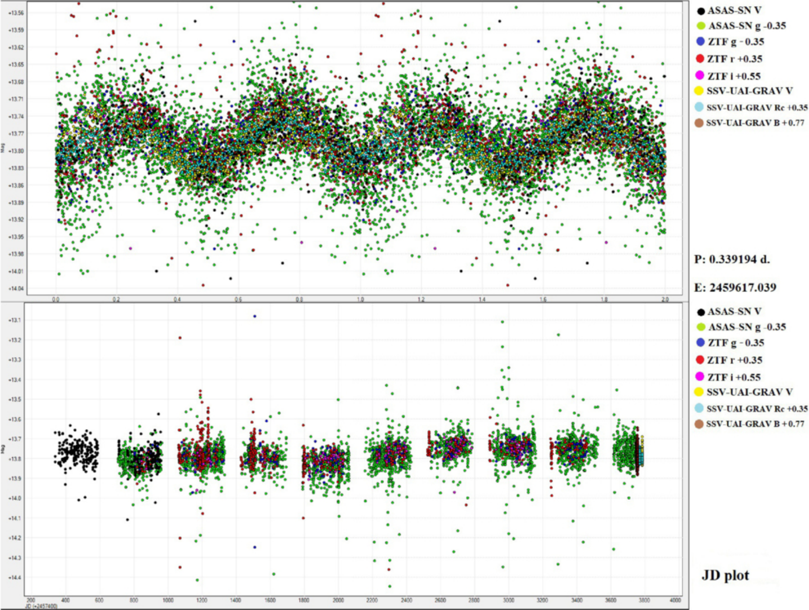
Figure 1. from Ivo Peretto et al 2026 Res. Notes AAS 10 doi:10.3847/2515-5172/aea215 https://dx.doi.org/10.3847/2515-5172/aea215 © 2026. The Author(s). Published by the American Astronomical Society.
