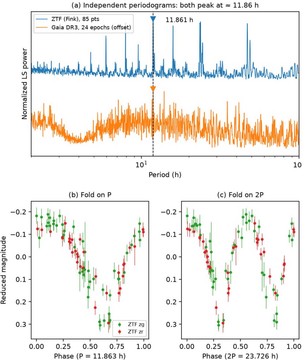
Figure 1. from Ilia Belykh 2026 Res. Notes AAS 10 doi:10.3847/2515-5172/aea158 https://dx.doi.org/10.3847/2515-5172/aea158 © 2026. The Author(s). Published by the American Astronomical Society.
