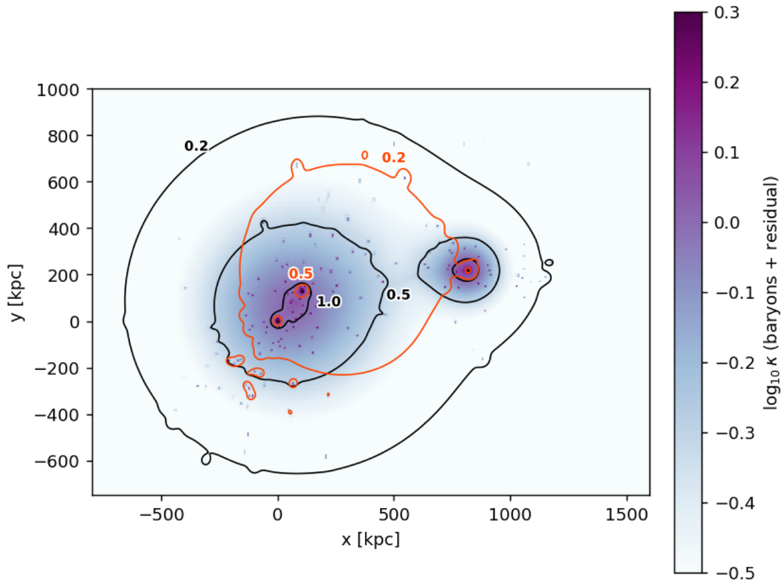
Figure 1. from Benoit Famaey 2026 Res. Notes AAS 10 doi:10.3847/2515-5172/ae9f45 https://dx.doi.org/10.3847/2515-5172/ae9f45 © 2026. The Author(s). Published by the American Astronomical Society.
