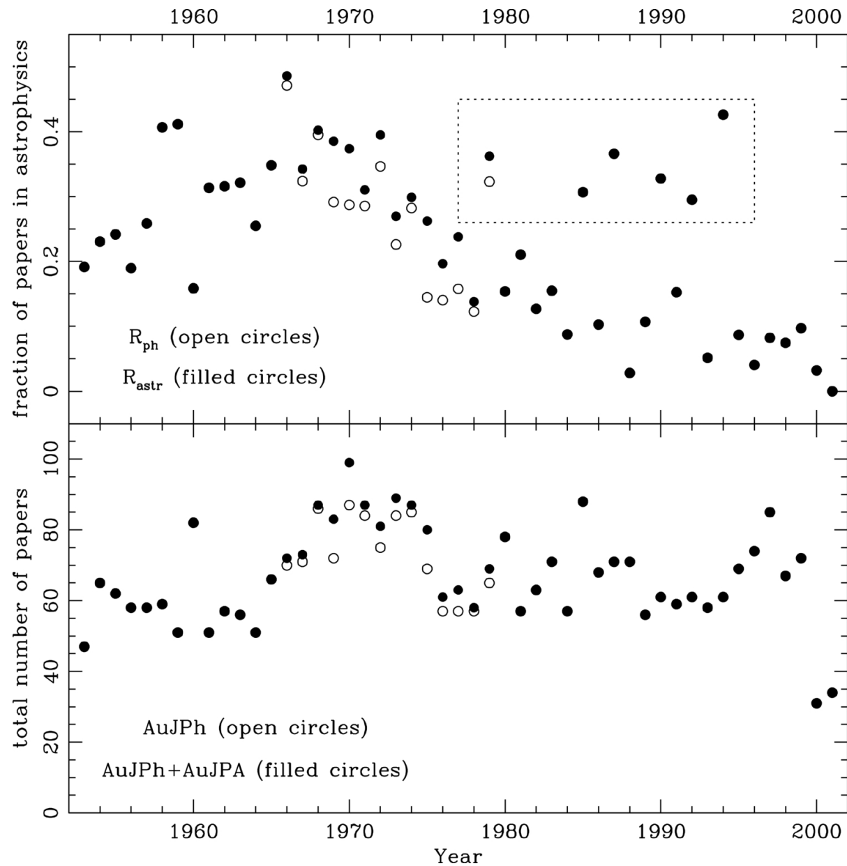
Figure 1. from Graeme H. Smith 2026 Res. Notes AAS 10 doi:10.3847/2515-5172/ae9cb5 https://dx.doi.org/10.3847/2515-5172/ae9cb5 © 2026. The Author(s). Published by the American Astronomical Society.
