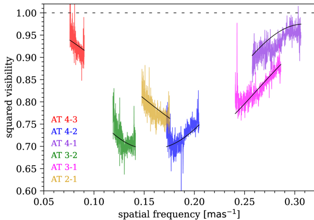
Figure 1. from Idel Waisberg et al 2026 Res. Notes AAS 10 doi:10.3847/2515-5172/ae9a71 https://dx.doi.org/10.3847/2515-5172/ae9a71 © 2026. The Author(s). Published by the American Astronomical Society.
