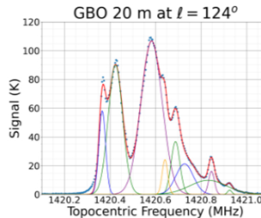
c. GBO 20 m Telescope Spectrum at l = 124^\circ .
