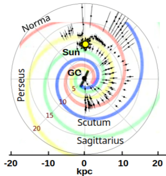
b. Map from the horn telescope data plotted over a theoretical model.
