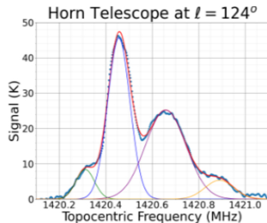
a. Horn Telescope Spectrum at l = 124^\circ .
