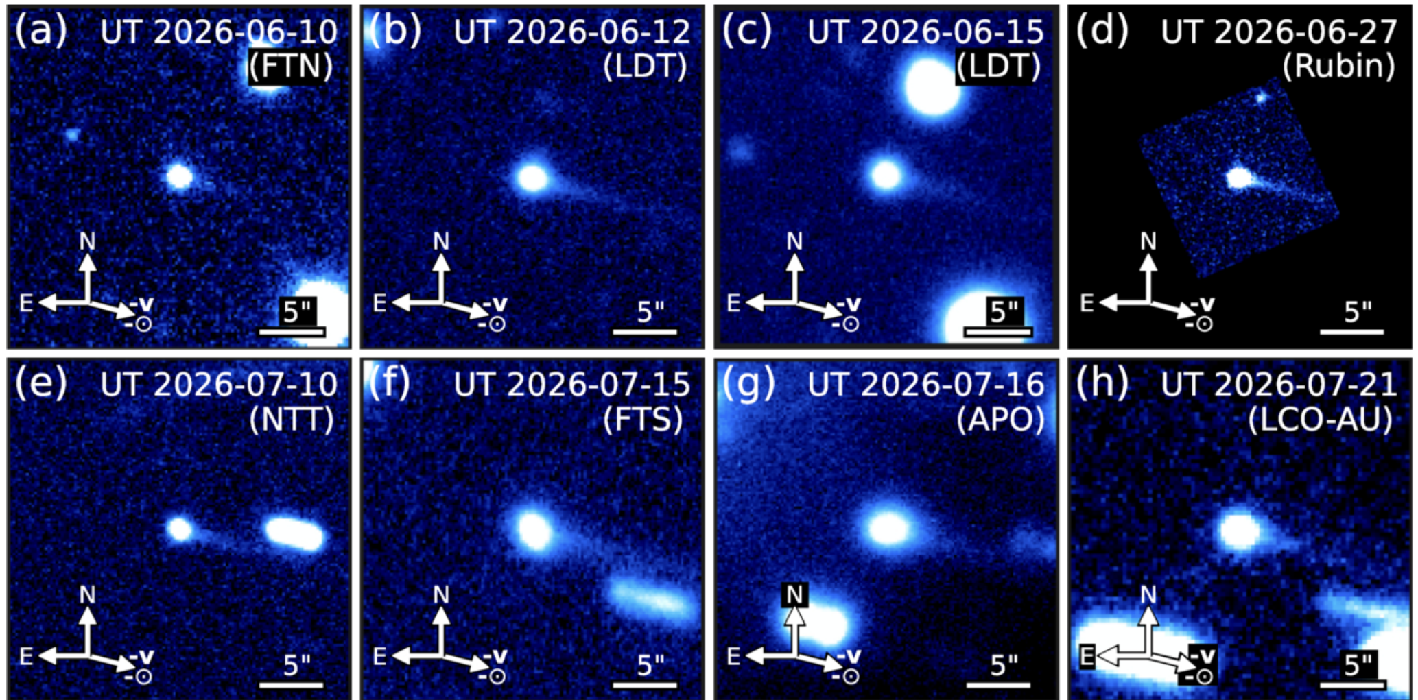
Figure 1. from Henry H. Hsieh et al 2026 Res. Notes AAS 10 doi:10.3847/2515-5172/ae954a https://dx.doi.org/10.3847/2515-5172/ae954a © 2026. The Author(s). Published by the American Astronomical Society.
