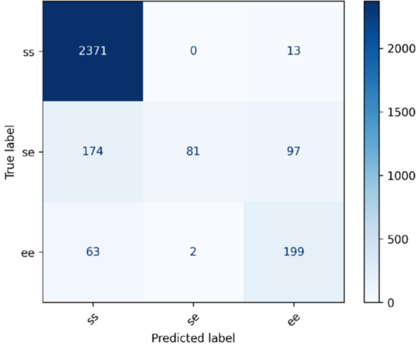
Confusion Matrix — N20000, S-S 50%, S-E 25%, E-E 25%
