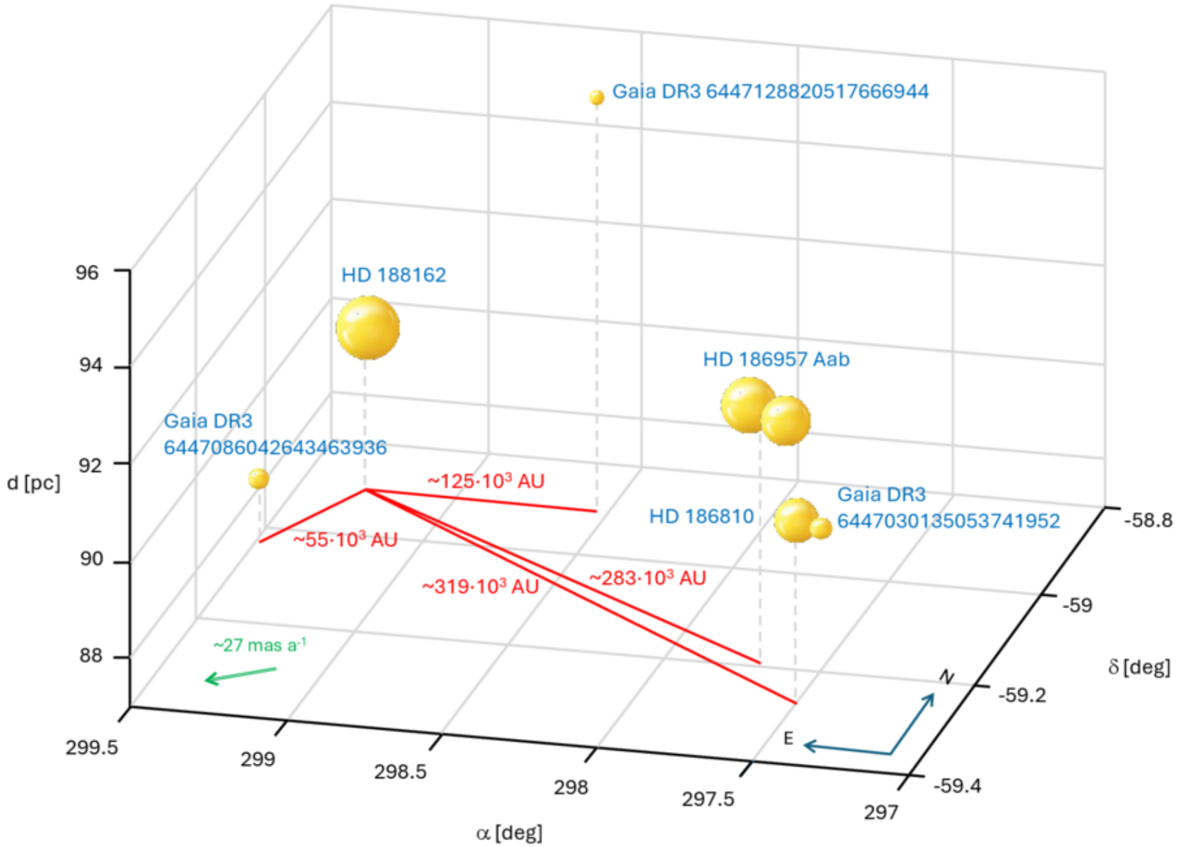
Figure 1. from Javier González-Payo 2026 Res. Notes AAS 10 doi:10.3847/2515-5172/ae86f4 https://dx.doi.org/10.3847/2515-5172/ae86f4 © 2026. The Author(s). Published by the American Astronomical Society.
