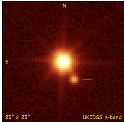
(a) UKIDSS LAS image
