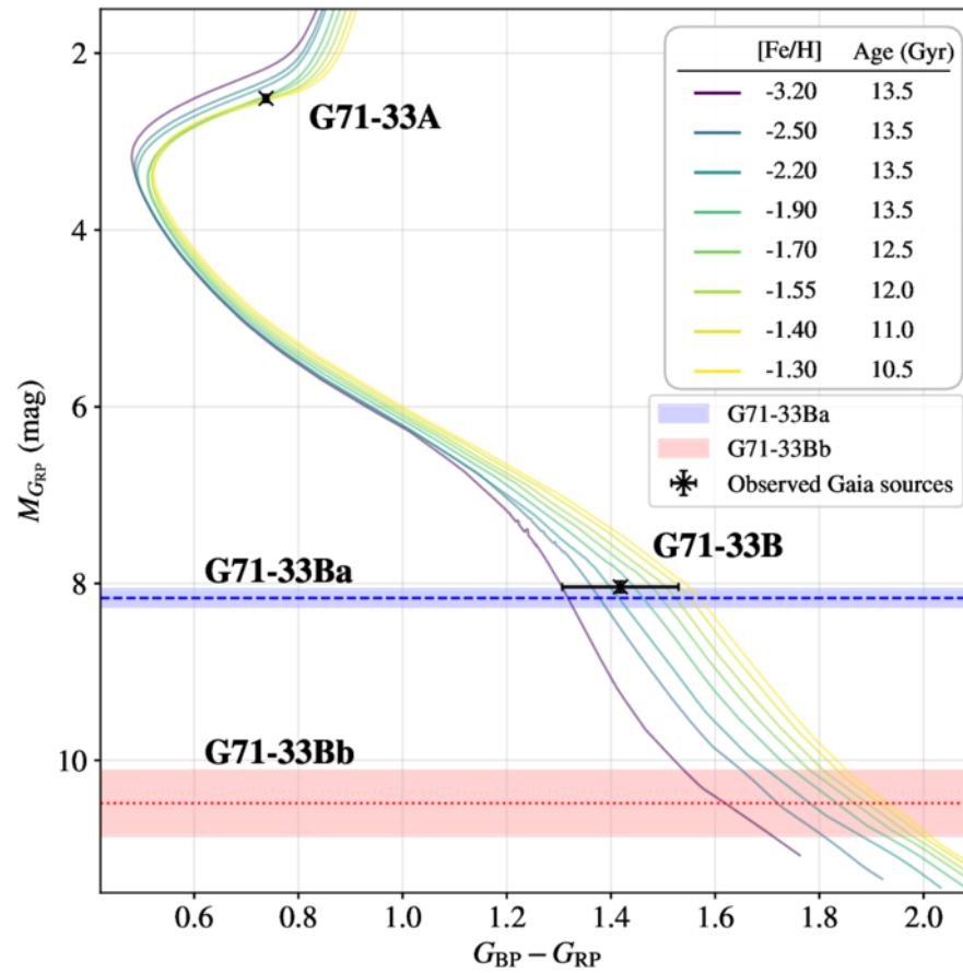
(c) HR diagram
