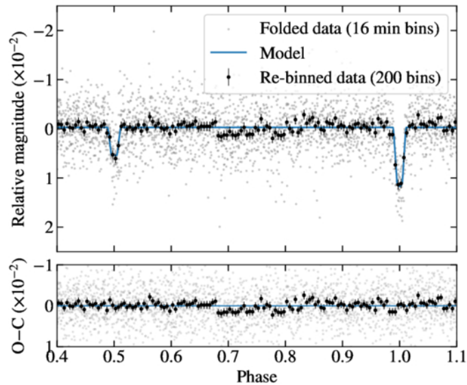
(b) Eclipse model
