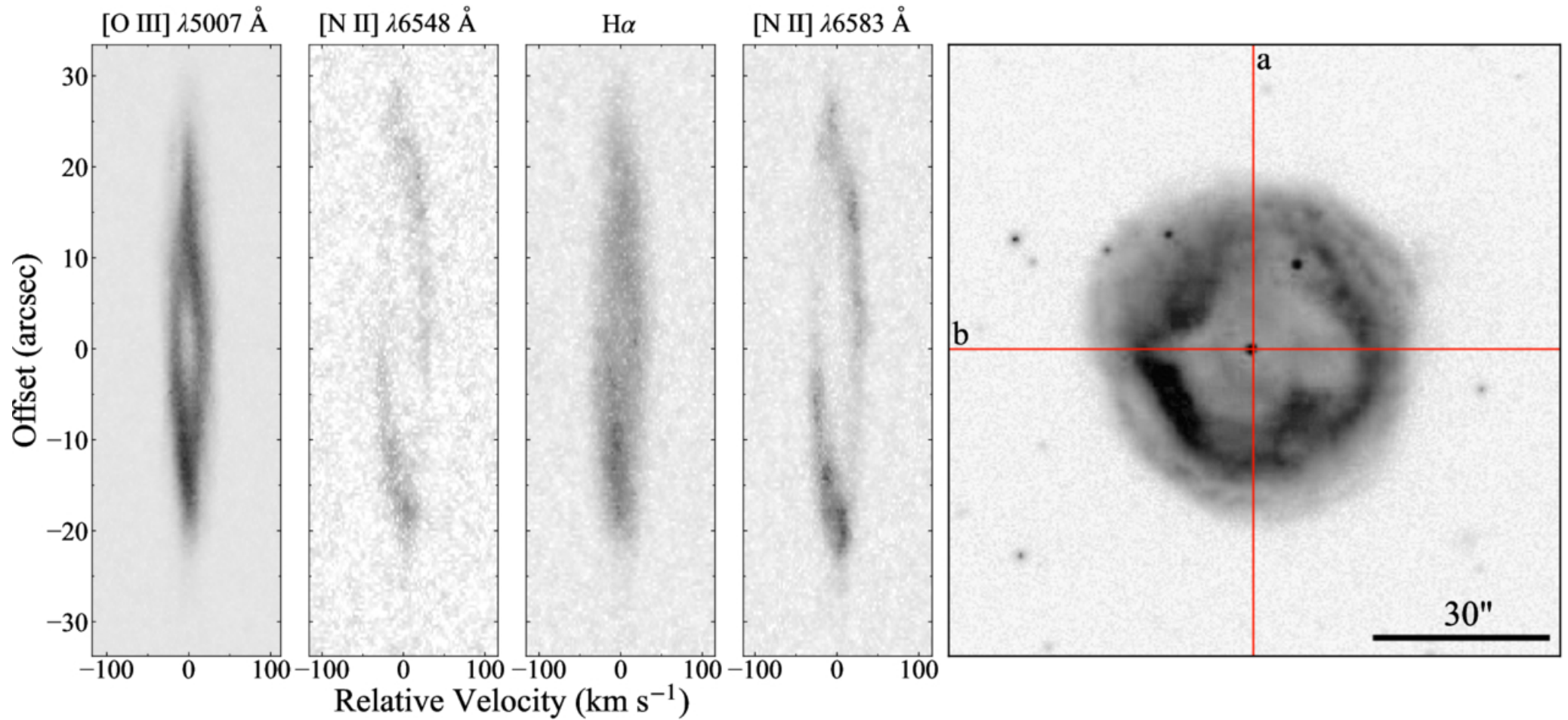
Figure 1. from M. Landa-Gomez et al 2026 Res. Notes AAS 10 doi:10.3847/2515-5172/ae83b1 https://dx.doi.org/10.3847/2515-5172/ae83b1 © 2026. The Author(s). Published by the American Astronomical Society.
