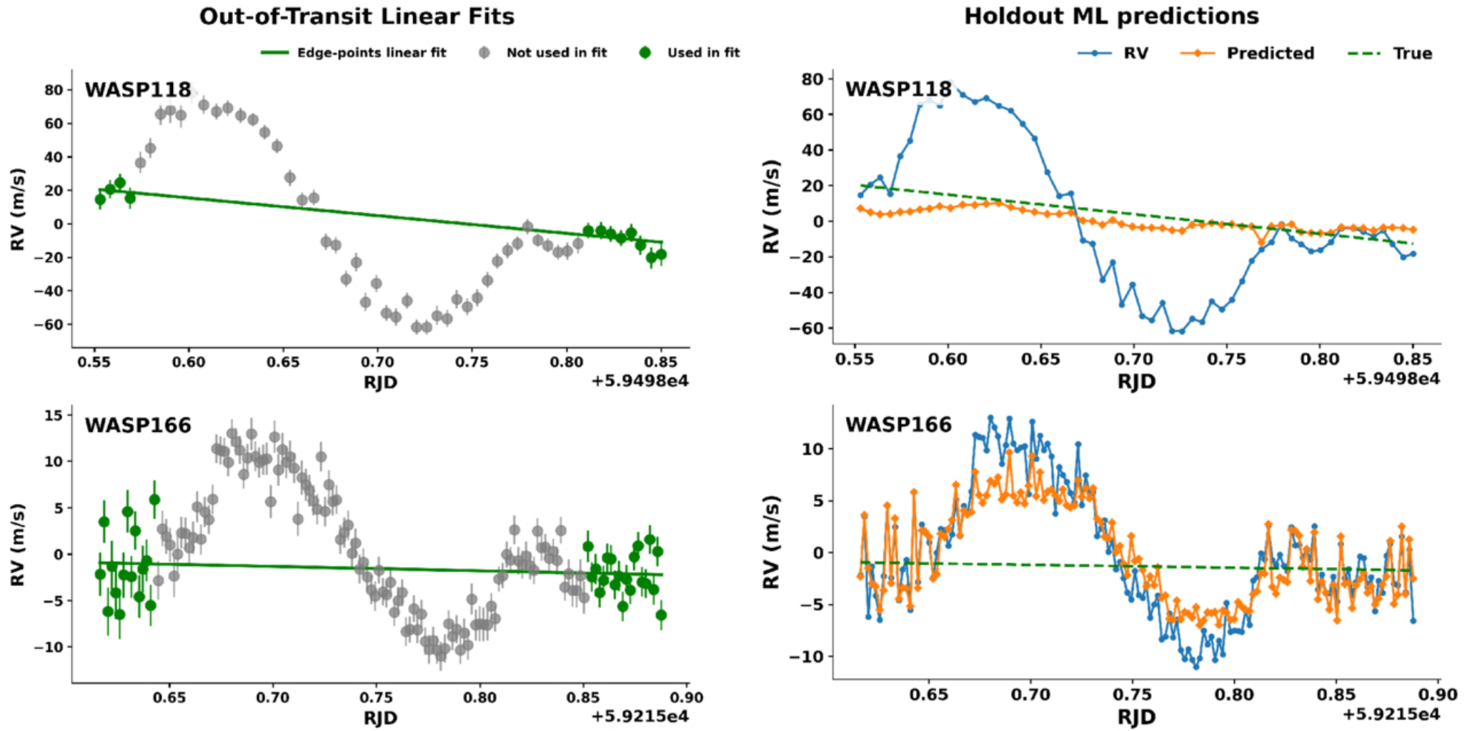
Figure 1. from Vardan Adibekyan et al 2026 Res. Notes AAS 10 doi:10.3847/2515-5172/ae8391 https://dx.doi.org/10.3847/2515-5172/ae8391 © 2026. The Author(s). Published by the American Astronomical Society.
