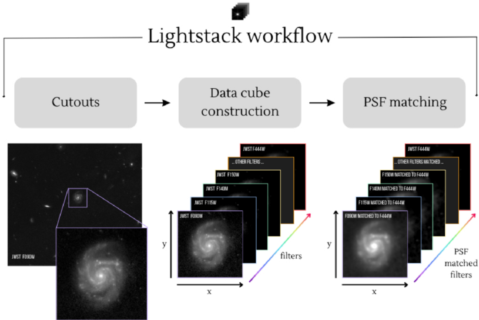
Figure 1. from Andressa Wille et al 2026 Res. Notes AAS 10 doi:10.3847/2515-5172/ae7c78 https://dx.doi.org/10.3847/2515-5172/ae7c78 © 2026. The Author(s). Published by the American Astronomical Society.
