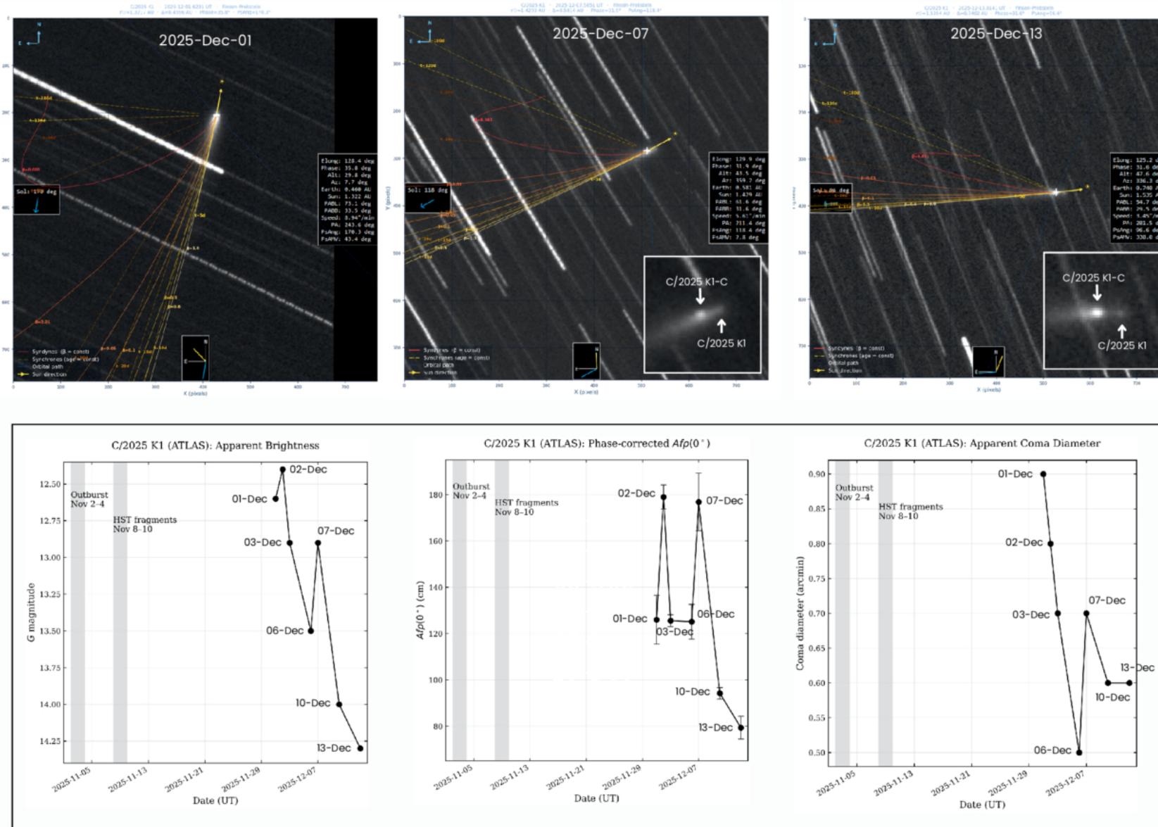
Figure 1. from Teerasak Thaluang 2026 Res. Notes AAS 10 doi:10.3847/2515-5172/ae7a6d https://dx.doi.org/10.3847/2515-5172/ae7a6d © 2026. The Author(s). Published by the American Astronomical Society.
