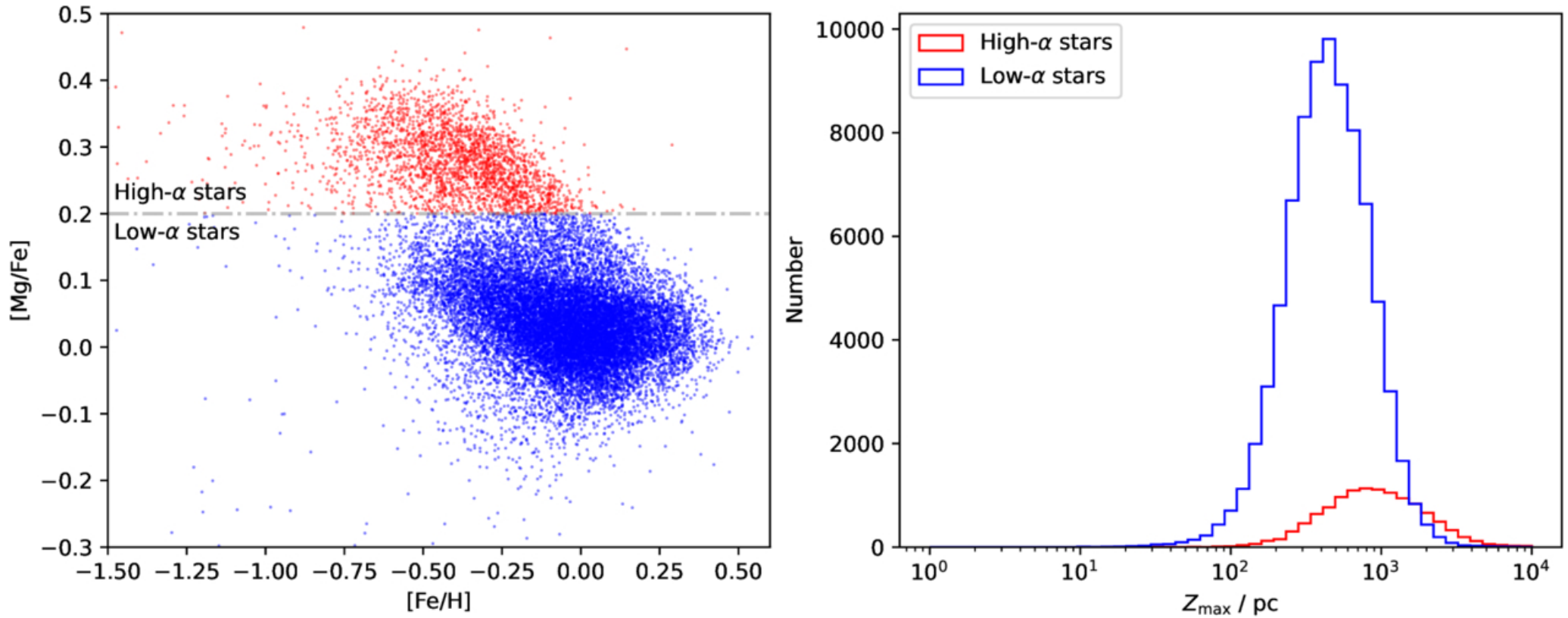
Figure 1. from Matthew J. Hopkins et al 2026 Res. Notes AAS 10 doi:10.3847/2515-5172/ae73fd https://dx.doi.org/10.3847/2515-5172/ae73fd © 2026. The Author(s). Published by the American Astronomical Society.
