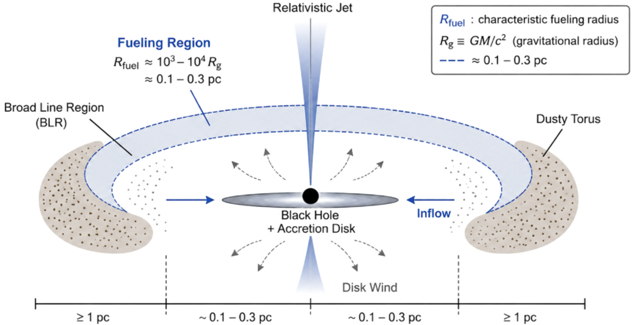
Figure 1. from David Garofalo 2026 Res. Notes AAS 10 doi:10.3847/2515-5172/ae6fb9 https://dx.doi.org/10.3847/2515-5172/ae6fb9 © 2026. The Author(s). Published by the American Astronomical Society.
