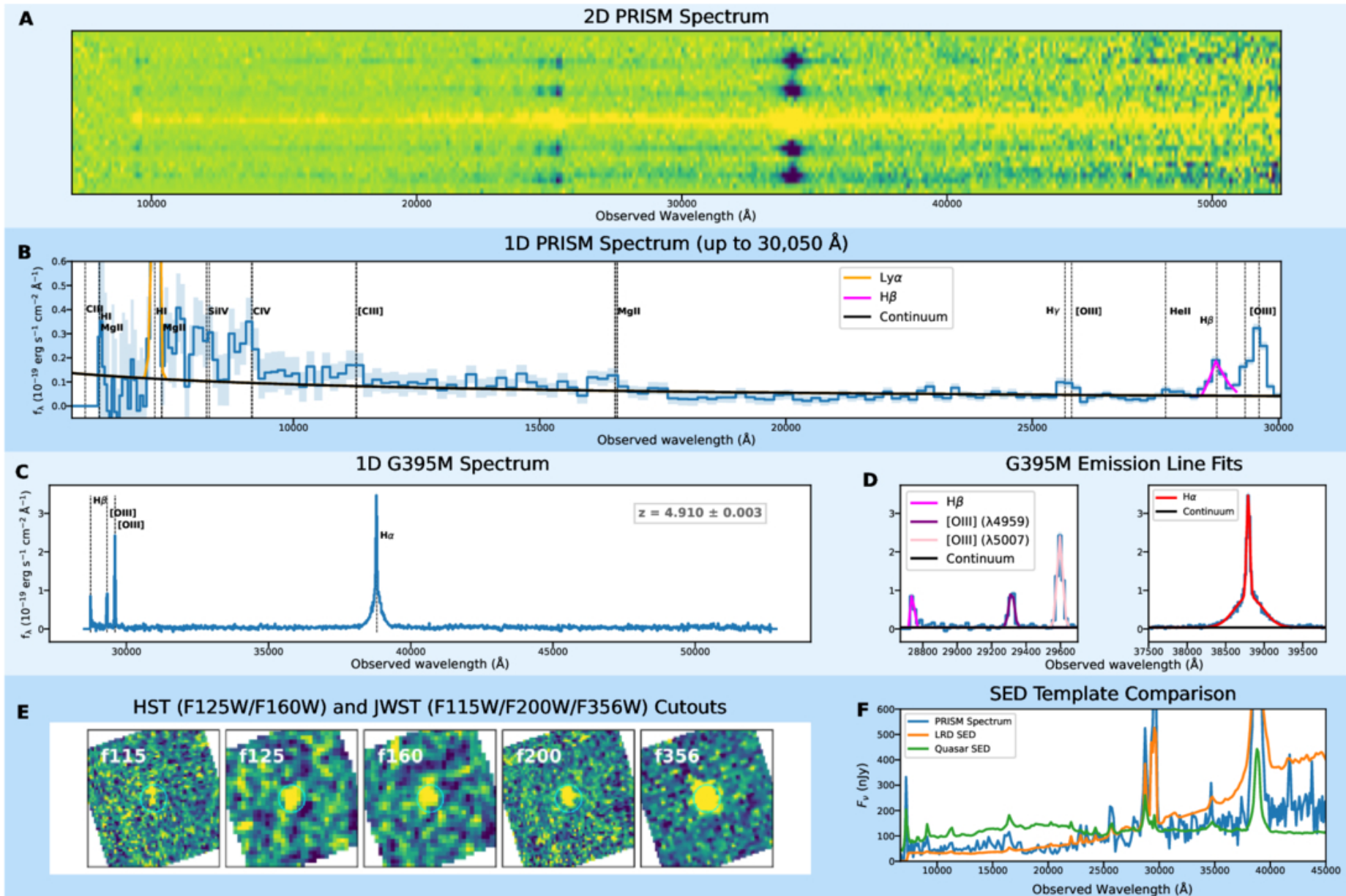
Figure 1. from Elaina Malczewski et al 2026 Res. Notes AAS 10 doi:10.3847/2515-5172/ae6b88 https://dx.doi.org/10.3847/2515-5172/ae6b88 © 2026. The Author(s). Published by the American Astronomical Society.
