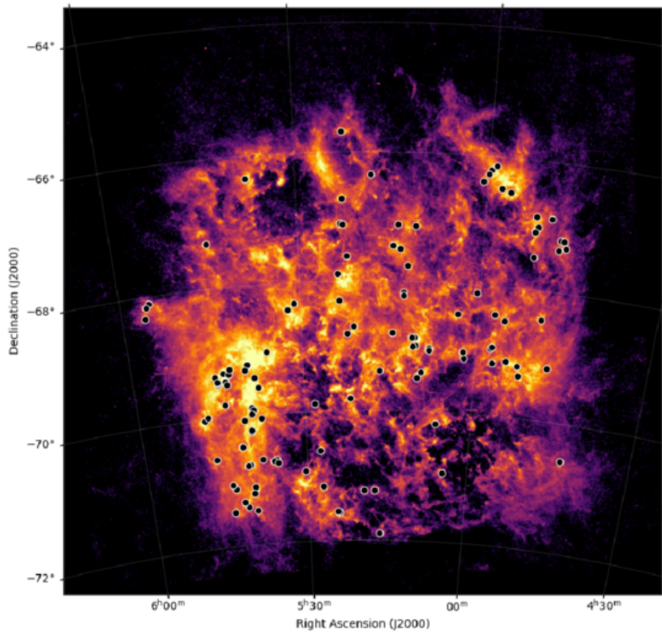
Figure 1. from Dia Kalra et al 2026 Res. Notes AAS 10 doi:10.3847/2515-5172/ae67f3 https://dx.doi.org/10.3847/2515-5172/ae67f3 © 2026. The Author(s). Published by the American Astronomical Society.
