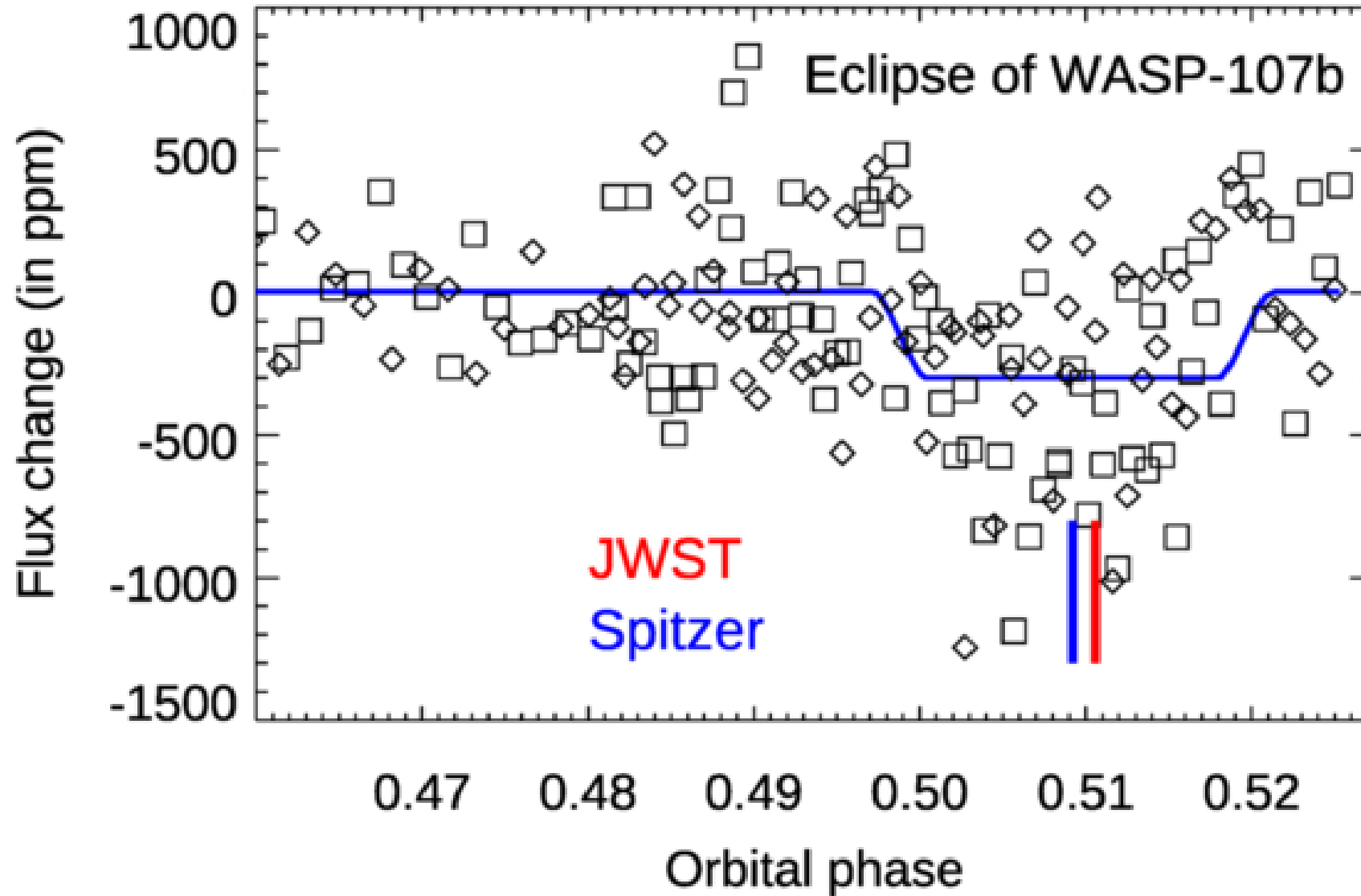
Figure 1. from Drake Deming and Laura Kreidberg 2026 Res. Notes AAS 10 doi:10.3847/2515-5172/ae6661 https://dx.doi.org/10.3847/2515-5172/ae6661 © 2026. The Author(s). Published by the American Astronomical Society.
