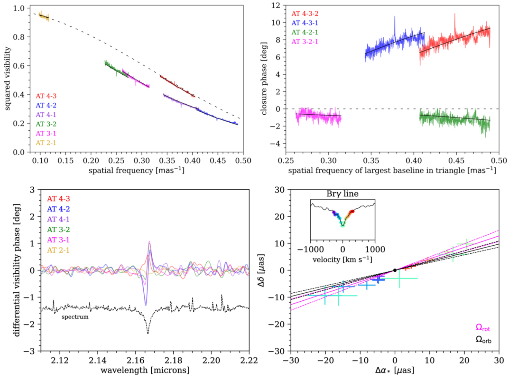
Figure 1. from Idel Waisberg et al 2026 Res. Notes AAS 10 doi:10.3847/2515-5172/ae5a98 https://dx.doi.org/10.3847/2515-5172/ae5a98 © 2026. The Author(s). Published by the American Astronomical Society.
