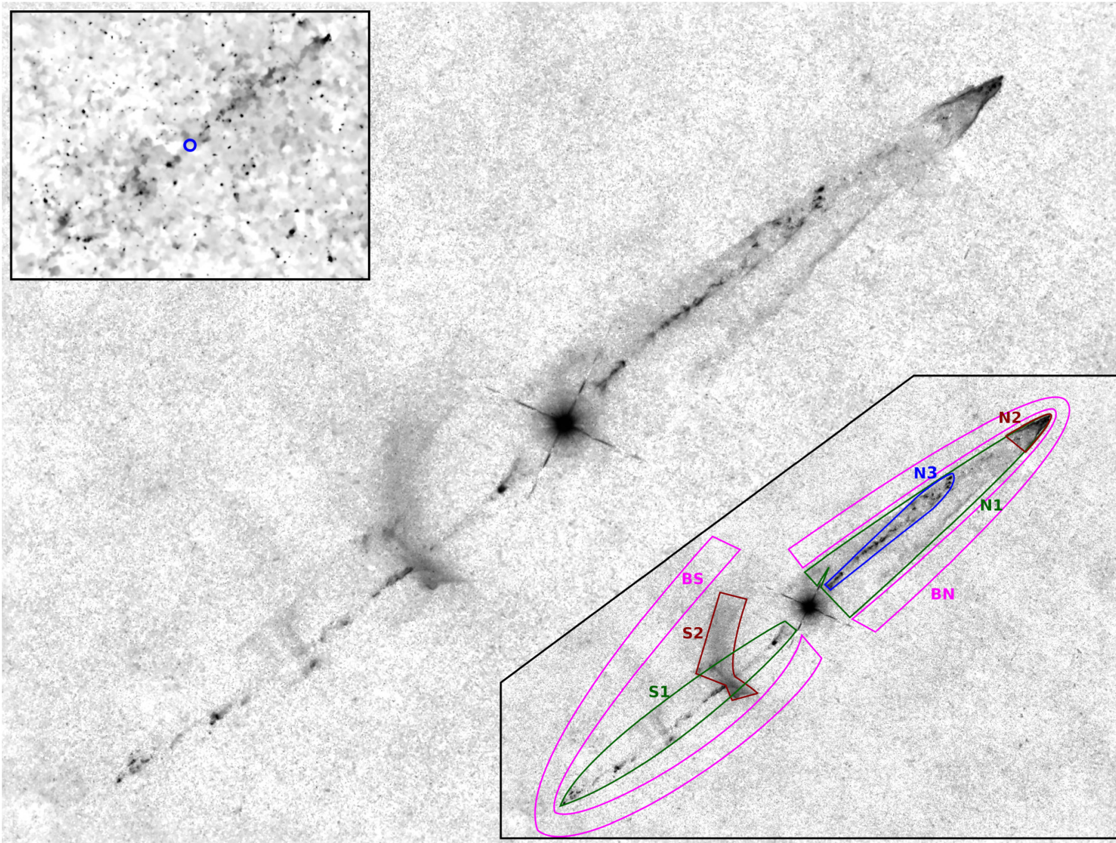
Figure 1. from Stefan Ziegenbalg 2024 Res. Notes AAS 8 doi:10.3847/2515-5172/ad9478 https://dx.doi.org/10.3847/2515-5172/ad9478 © 2024. The Author(s). Published by the American Astronomical Society.
