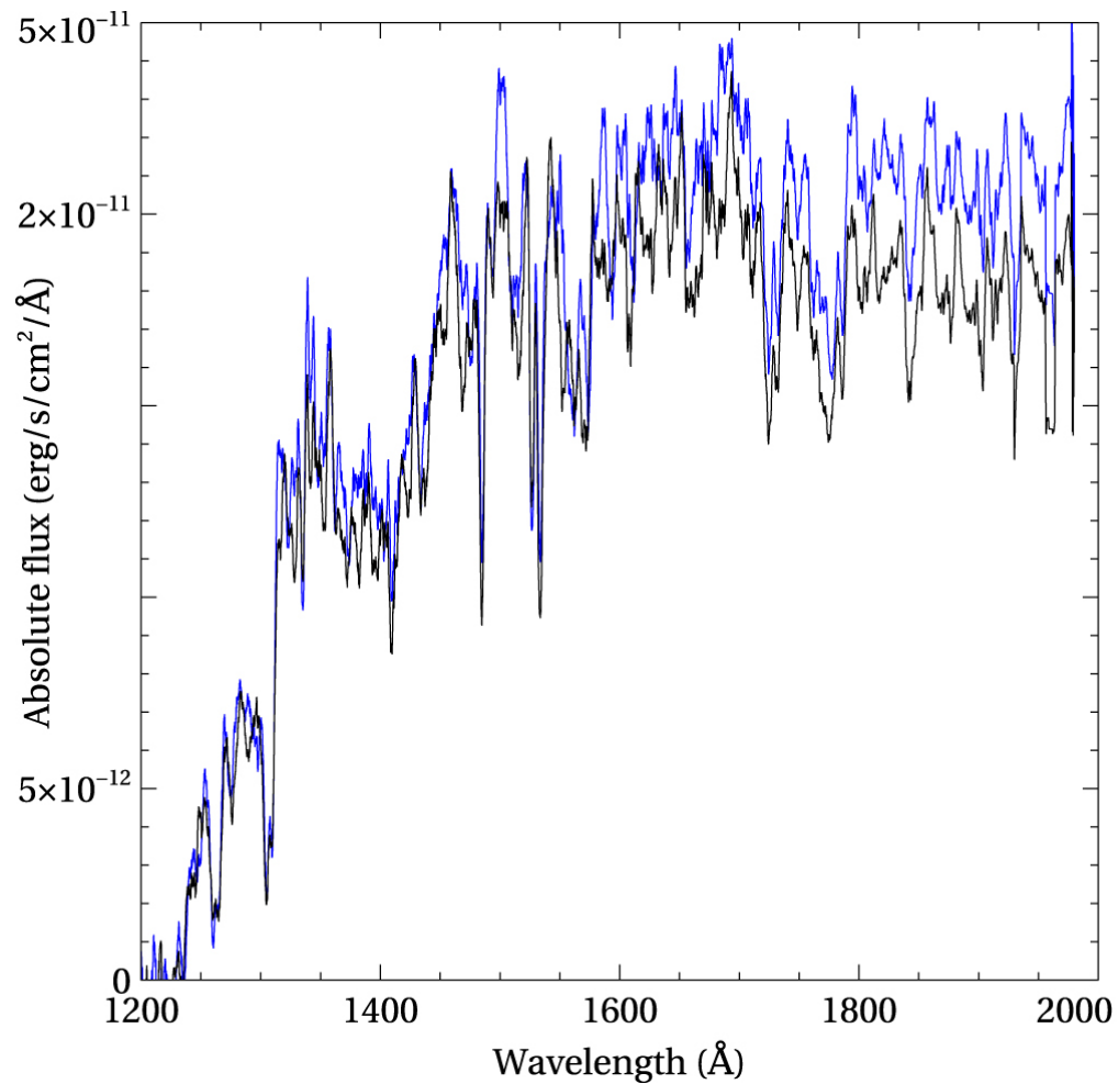
Figure 1. from Richard Monier and Patricia Lampens 2021 Res. Notes AAS 5 doi:10.3847/2515-5172/ac3427 https://dx.doi.org/10.3847/2515-5172/ac3427 © 2021. The Author(s). Published by the American Astronomical Society.
