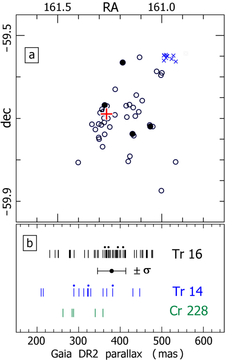
Figure 1. from Gaia, Trumpler 16, and Eta Carinae null 2018 RNAAS 2 133 doi:10.3847/2515-5172/aad63c https://dx.doi.org/10.3847/2515-5172/aad63c © 2018. The American Astronomical Society. All rights reserved.
