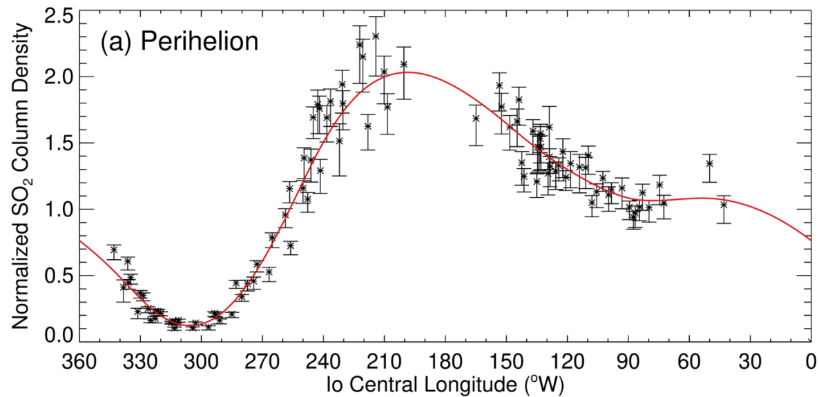
Figure 4. from Rohini S. Giles et al 2026 Planet. Sci. J. 7 doi:10.3847/PSJ/aeb269 https://dx.doi.org/10.3847/PSJ/aeb269 © 2026. The Author(s). Published by the American Astronomical Society.
