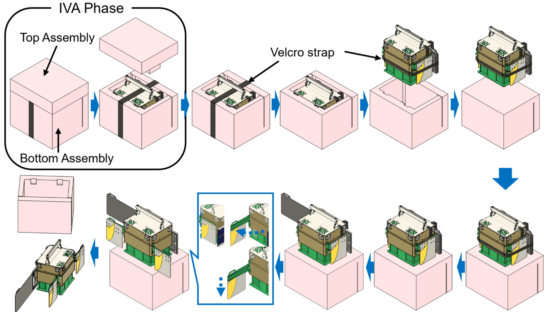
Figure 4. from Makito Kobayashi et al 2026 Planet. Sci. J. 7 doi:10.3847/PSJ/aeaff9 https://dx.doi.org/10.3847/PSJ/aeaff9 © 2026. The Author(s). Published by the American Astronomical Society.
