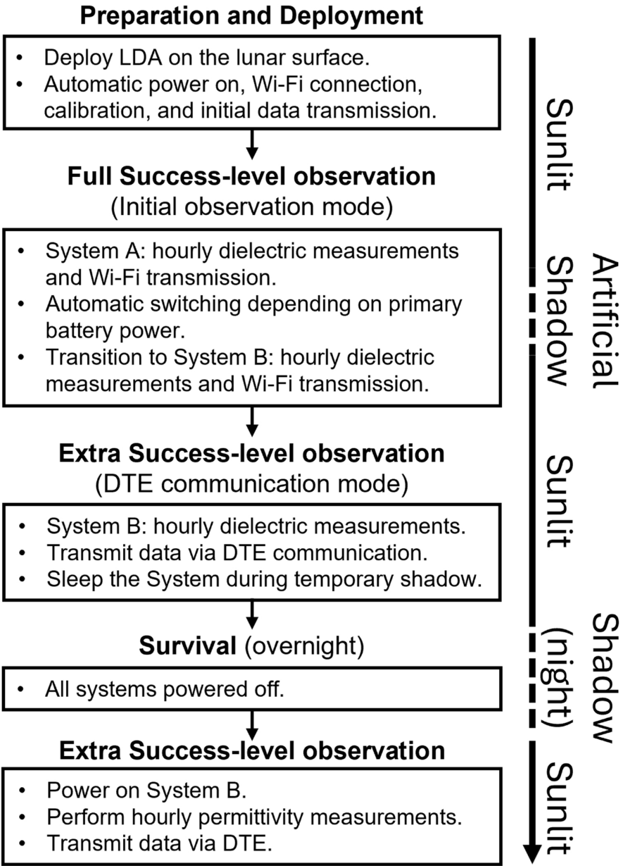
Figure 3. from Makito Kobayashi et al 2026 Planet. Sci. J. 7 doi:10.3847/PSJ/aeaff9 https://dx.doi.org/10.3847/PSJ/aeaff9 © 2026. The Author(s). Published by the American Astronomical Society.
