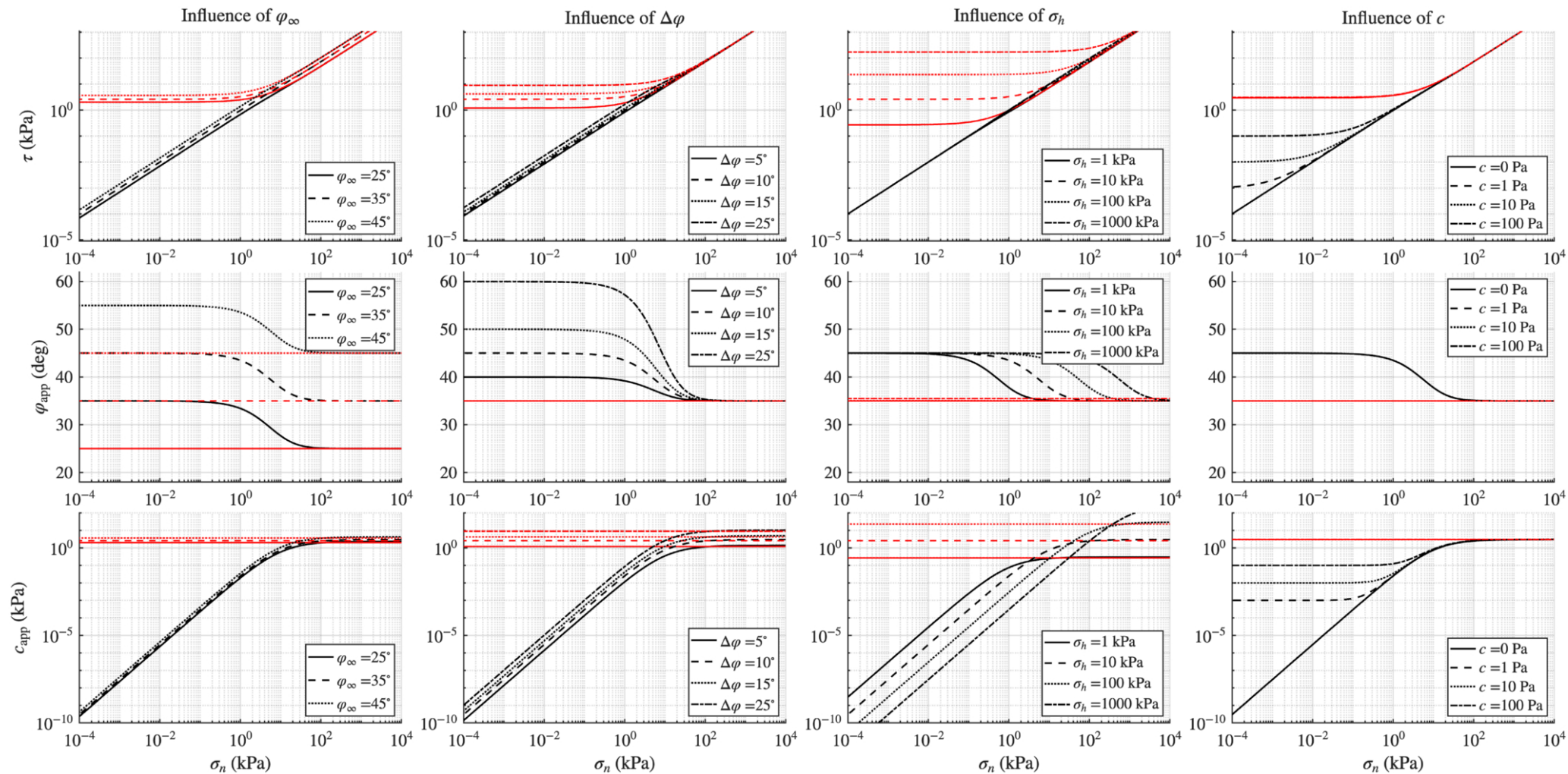
Figure 4. from Naomi Murdoch 2026 Planet. Sci. J. 7 doi:10.3847/PSJ/aeaa37 https://dx.doi.org/10.3847/PSJ/aeaa37 © 2026. The Author(s). Published by the American Astronomical Society.
