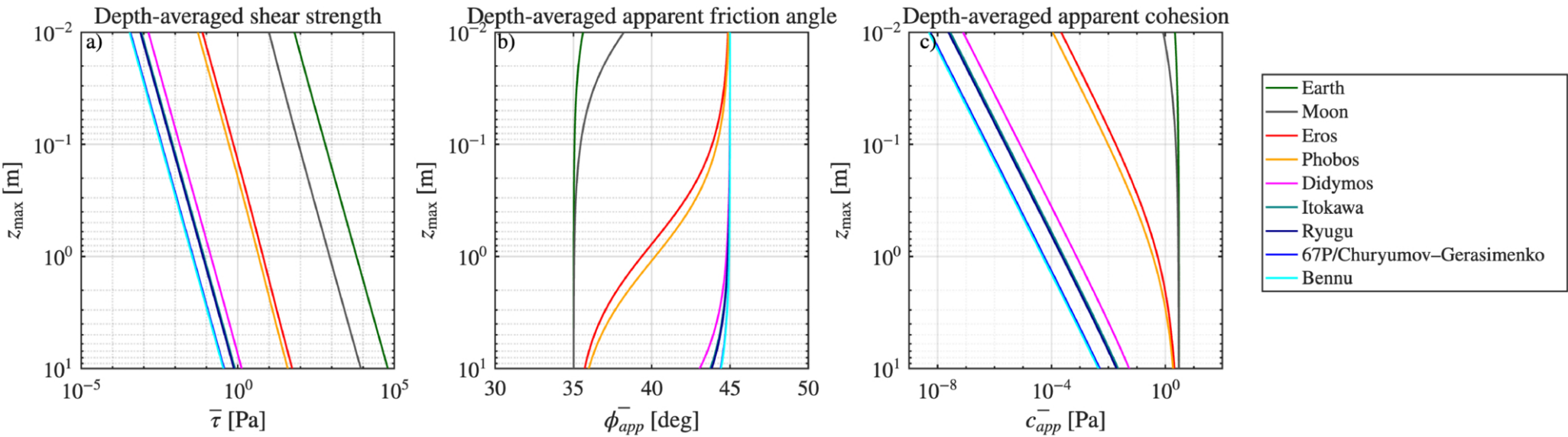
Figure 3. from Naomi Murdoch 2026 Planet. Sci. J. 7 doi:10.3847/PSJ/aeaa37 https://dx.doi.org/10.3847/PSJ/aeaa37 © 2026. The Author(s). Published by the American Astronomical Society.
