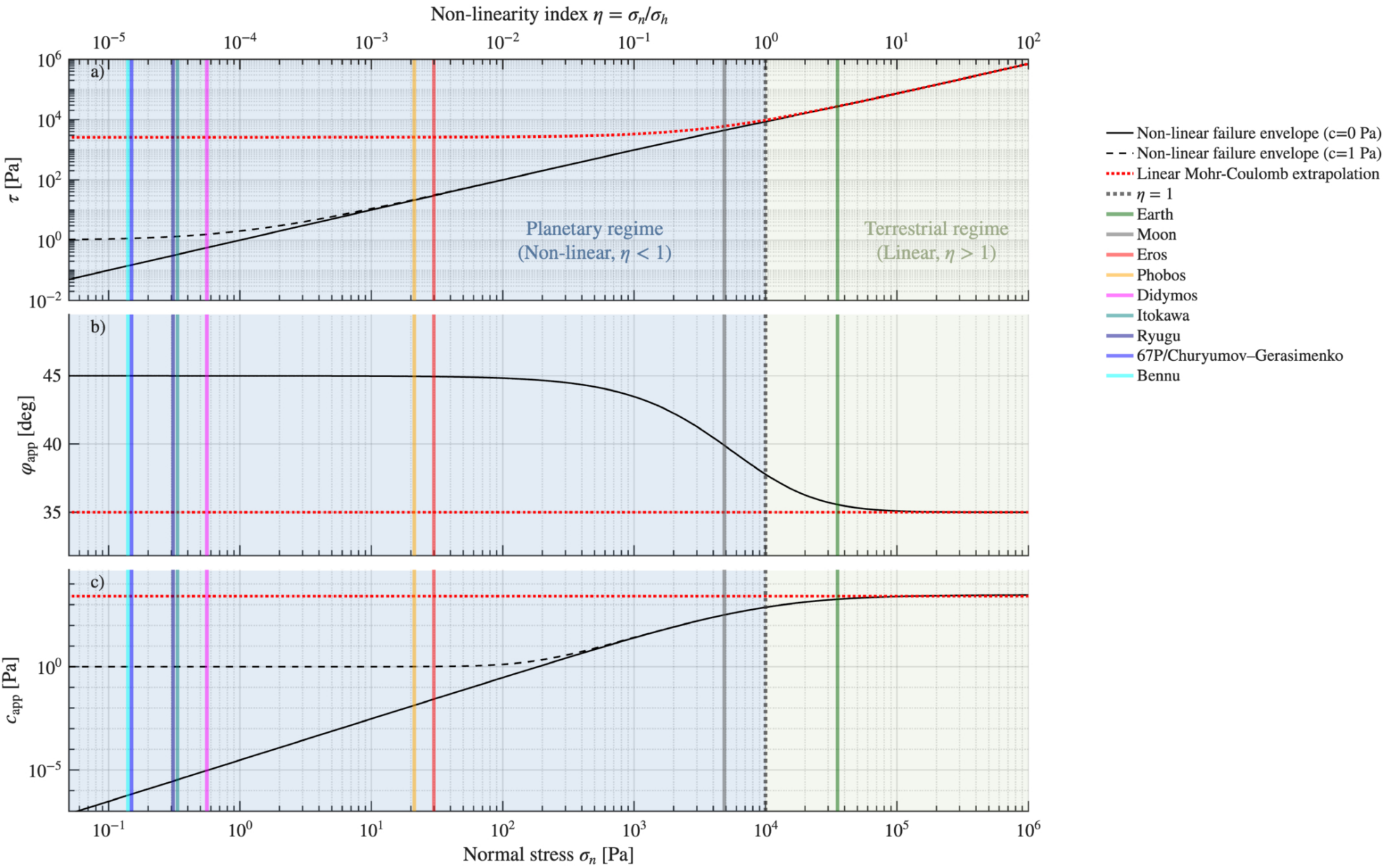
Figure 2. from Naomi Murdoch 2026 Planet. Sci. J. 7 doi:10.3847/PSJ/aeaa37 https://dx.doi.org/10.3847/PSJ/aeaa37 © 2026. The Author(s). Published by the American Astronomical Society.
