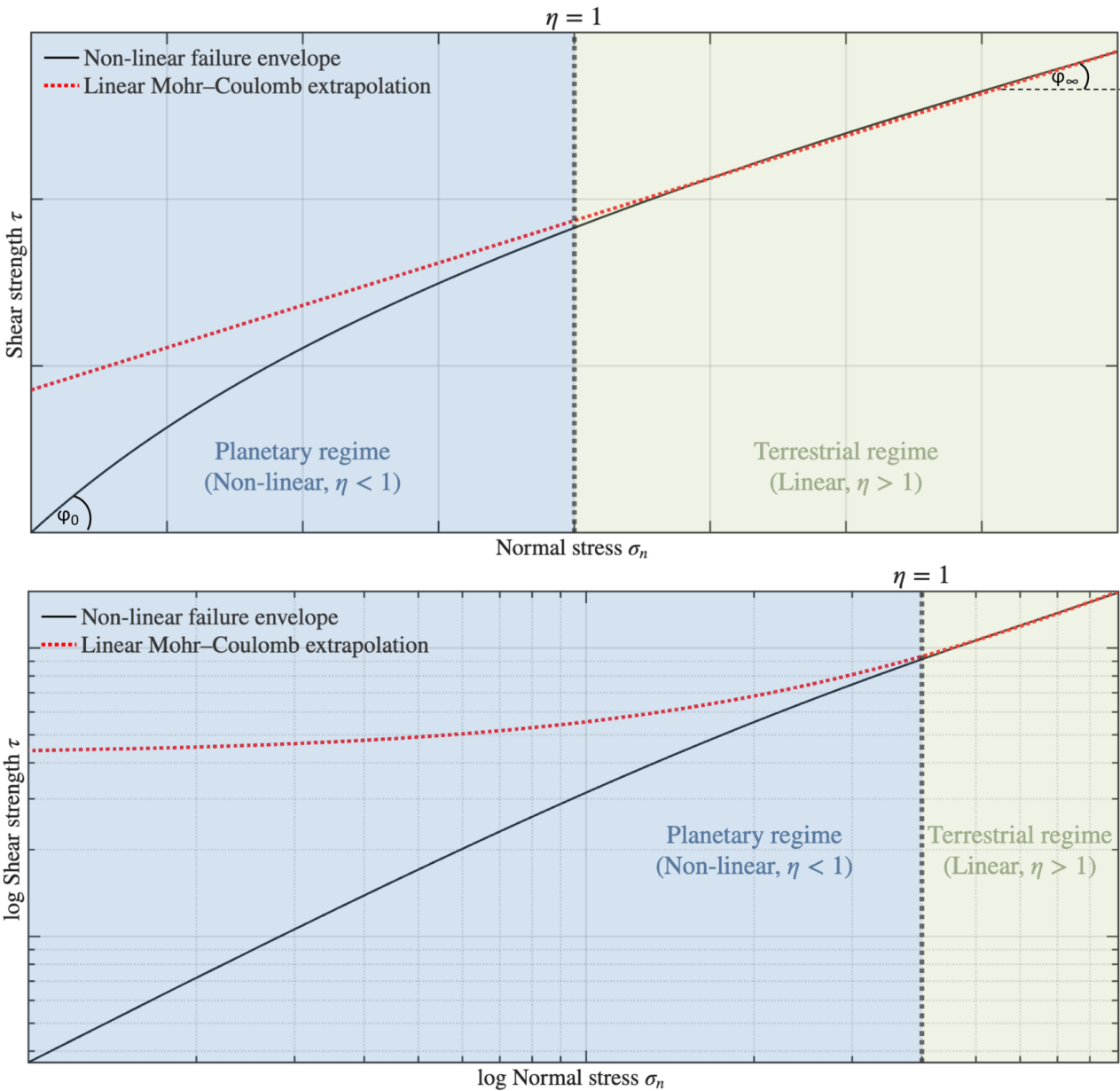
Figure 1. from Naomi Murdoch 2026 Planet. Sci. J. 7 doi:10.3847/PSJ/aeaa37 https://dx.doi.org/10.3847/PSJ/aeaa37 © 2026. The Author(s). Published by the American Astronomical Society.
