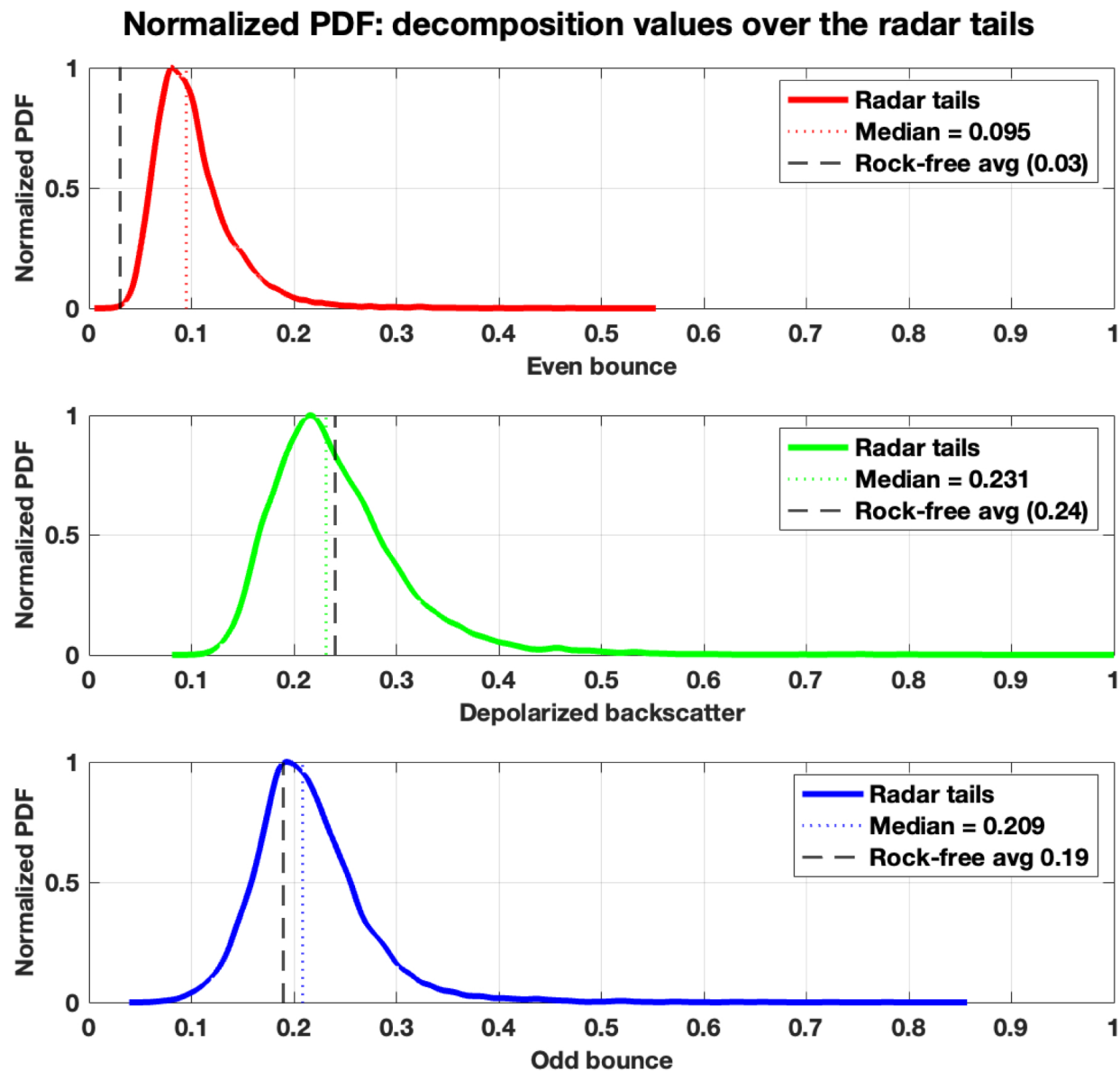
Figure 9. from Santa L. Pérez-Cortés et al 2026 Planet. Sci. J. 7 doi:10.3847/PSJ/aea98b https://dx.doi.org/10.3847/PSJ/aea98b © 2026. The Author(s). Published by the American Astronomical Society.
