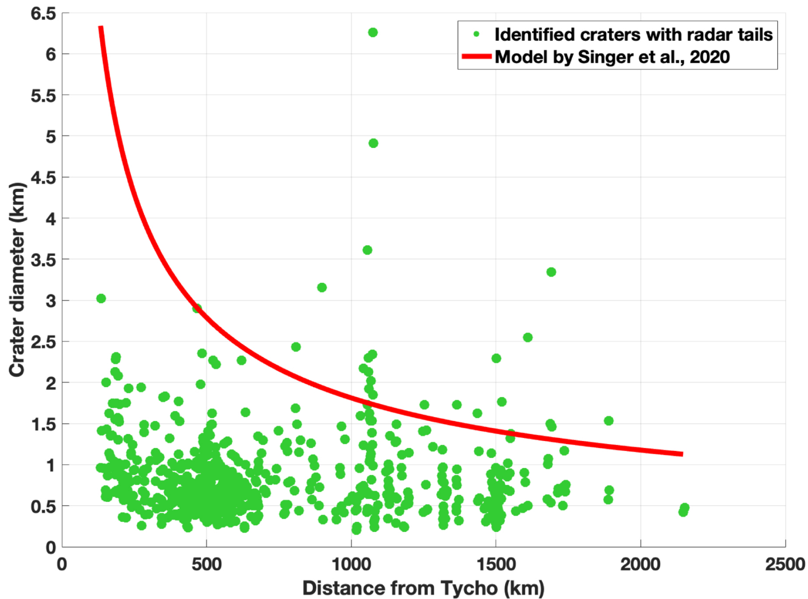
Figure 7. from Santa L. Pérez-Cortés et al 2026 Planet. Sci. J. 7 doi:10.3847/PSJ/aea98b https://dx.doi.org/10.3847/PSJ/aea98b © 2026. The Author(s). Published by the American Astronomical Society.
