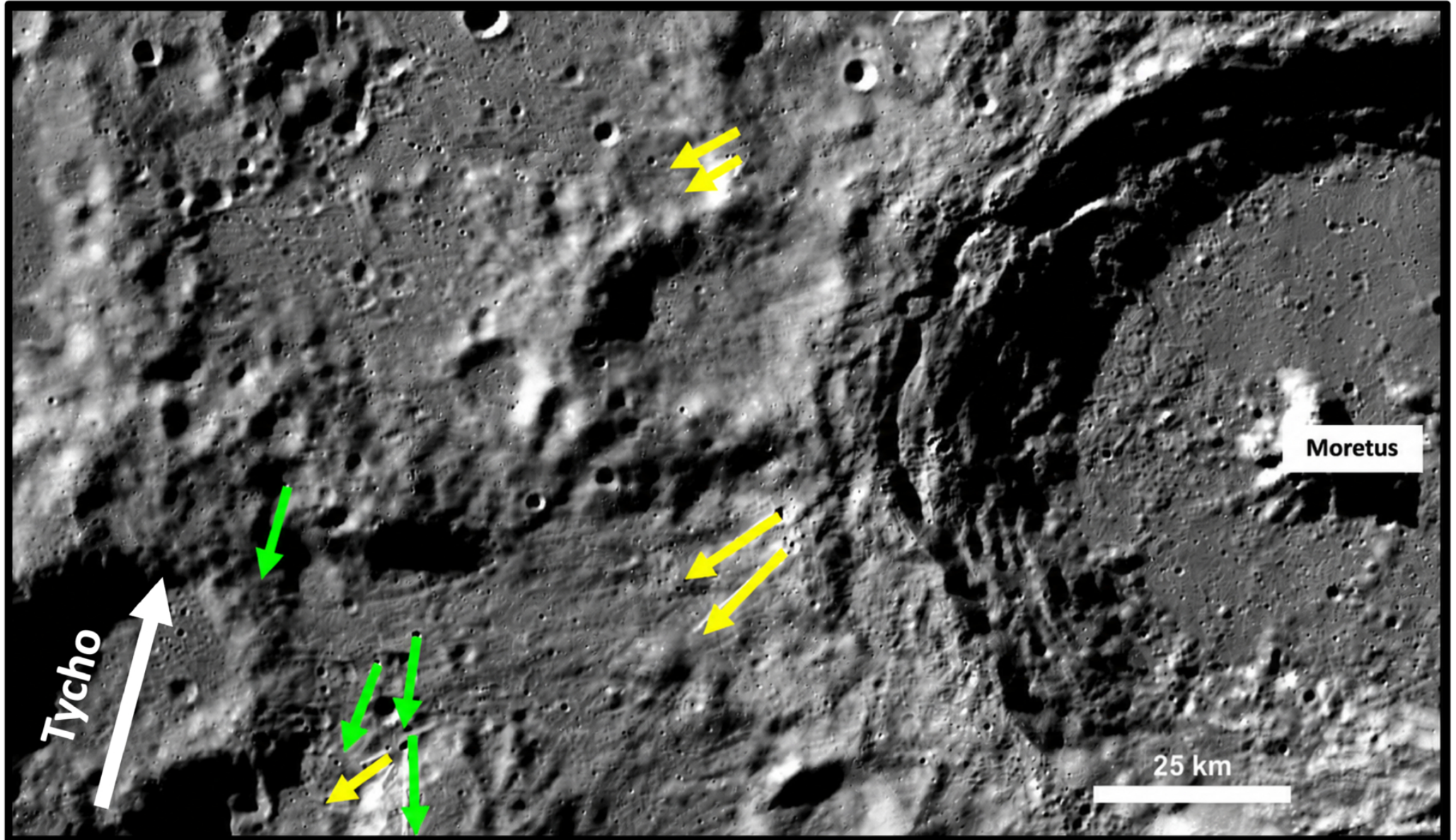
Figure 4. from Santa L. Pérez-Cortés et al 2026 Planet. Sci. J. 7 doi:10.3847/PSJ/aea98b https://dx.doi.org/10.3847/PSJ/aea98b © 2026. The Author(s). Published by the American Astronomical Society.
