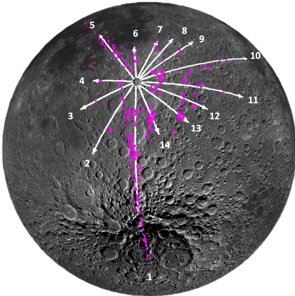
Figure 3. from Santa L. Pérez-Cortés et al 2026 Planet. Sci. J. 7 doi:10.3847/PSJ/aea98b https://dx.doi.org/10.3847/PSJ/aea98b © 2026. The Author(s). Published by the American Astronomical Society.
