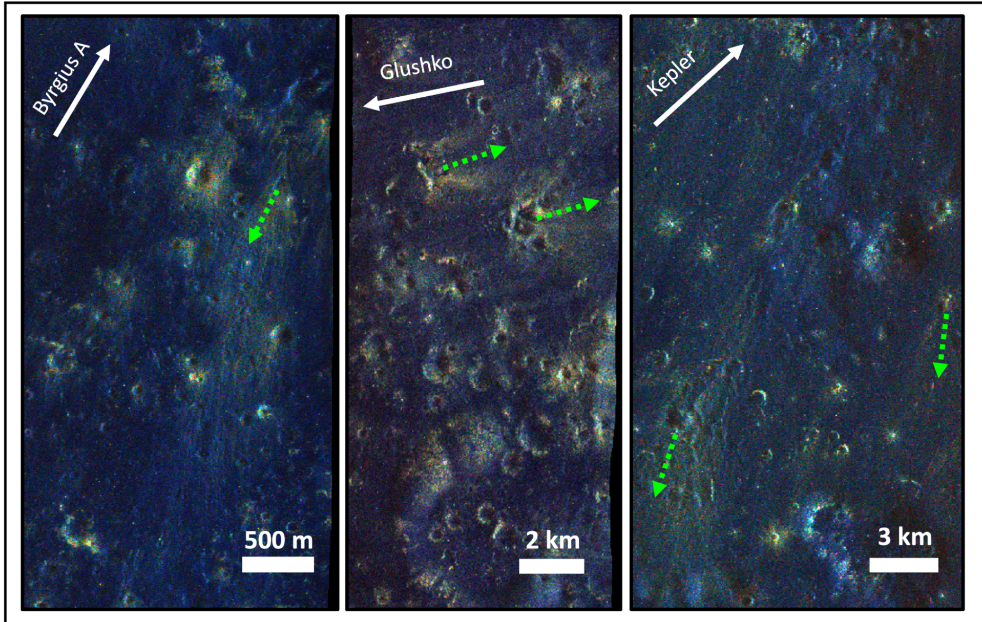
Figure 13. from Santa L. Pérez-Cortés et al 2026 Planet. Sci. J. 7 doi:10.3847/PSJ/aea98b https://dx.doi.org/10.3847/PSJ/aea98b © 2026. The Author(s). Published by the American Astronomical Society.
