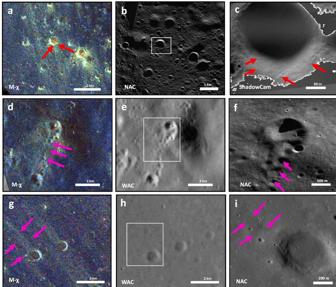
Figure 11. from Santa L. Pérez-Cortés et al 2026 Planet. Sci. J. 7 doi:10.3847/PSJ/aea98b https://dx.doi.org/10.3847/PSJ/aea98b © 2026. The Author(s). Published by the American Astronomical Society.
