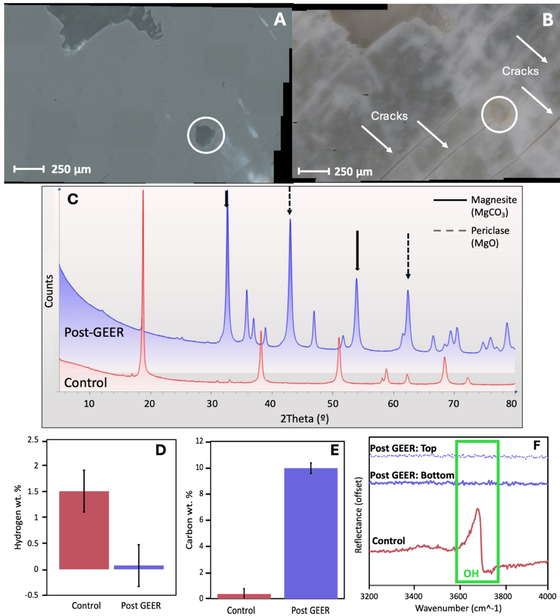
Figure 3. from Sara Taeko Port et al 2026 Planet. Sci. J. 7 doi:10.3847/PSJ/aea909 https://dx.doi.org/10.3847/PSJ/aea909 © 2026. The Author(s). Published by the American Astronomical Society.
