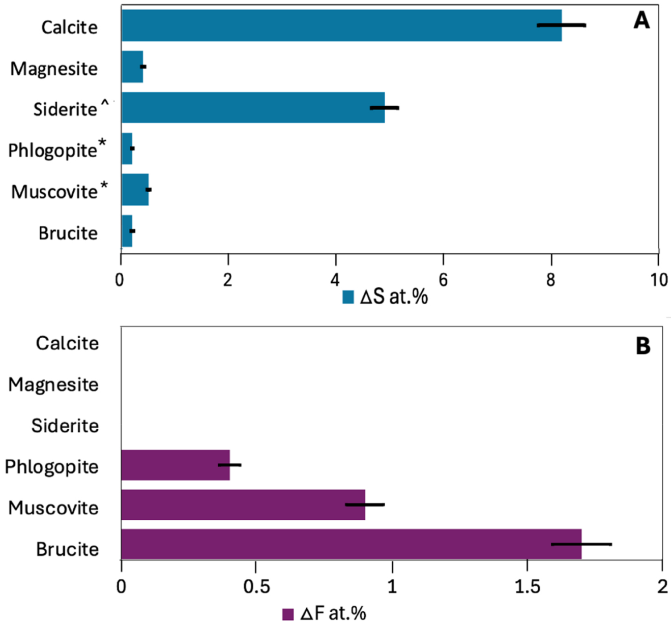
Figure 2. from Sara Taeko Port et al 2026 Planet. Sci. J. 7 doi:10.3847/PSJ/aea909 https://dx.doi.org/10.3847/PSJ/aea909 © 2026. The Author(s). Published by the American Astronomical Society.
