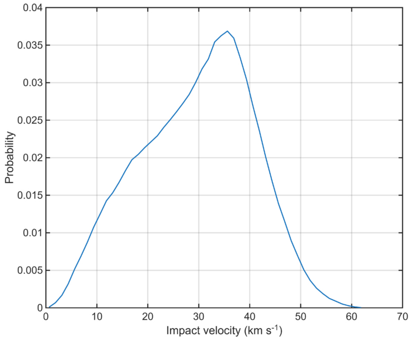
Figure 6. from Ian-Lin Lai et al 2026 Planet. Sci. J. 7 doi:10.3847/PSJ/aea848 https://dx.doi.org/10.3847/PSJ/aea848 © 2026. The Author(s). Published by the American Astronomical Society.
