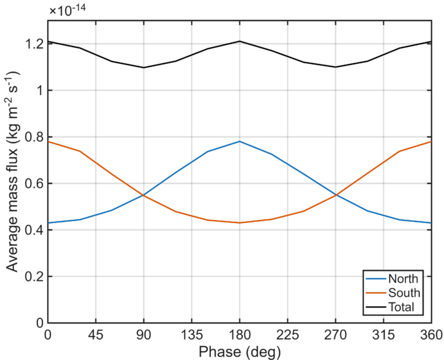
Figure 5. from Ian-Lin Lai et al 2026 Planet. Sci. J. 7 doi:10.3847/PSJ/aea848 https://dx.doi.org/10.3847/PSJ/aea848 © 2026. The Author(s). Published by the American Astronomical Society.
