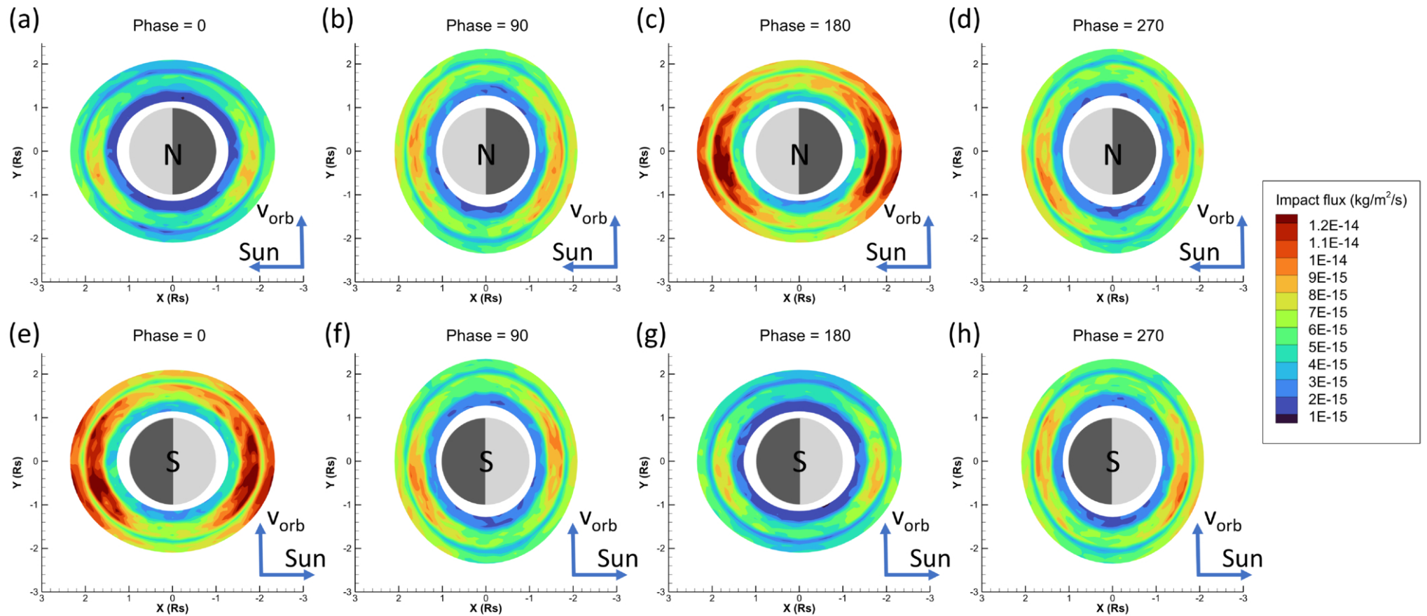
Figure 4. from Ian-Lin Lai et al 2026 Planet. Sci. J. 7 doi:10.3847/PSJ/aea848 https://dx.doi.org/10.3847/PSJ/aea848 © 2026. The Author(s). Published by the American Astronomical Society.
