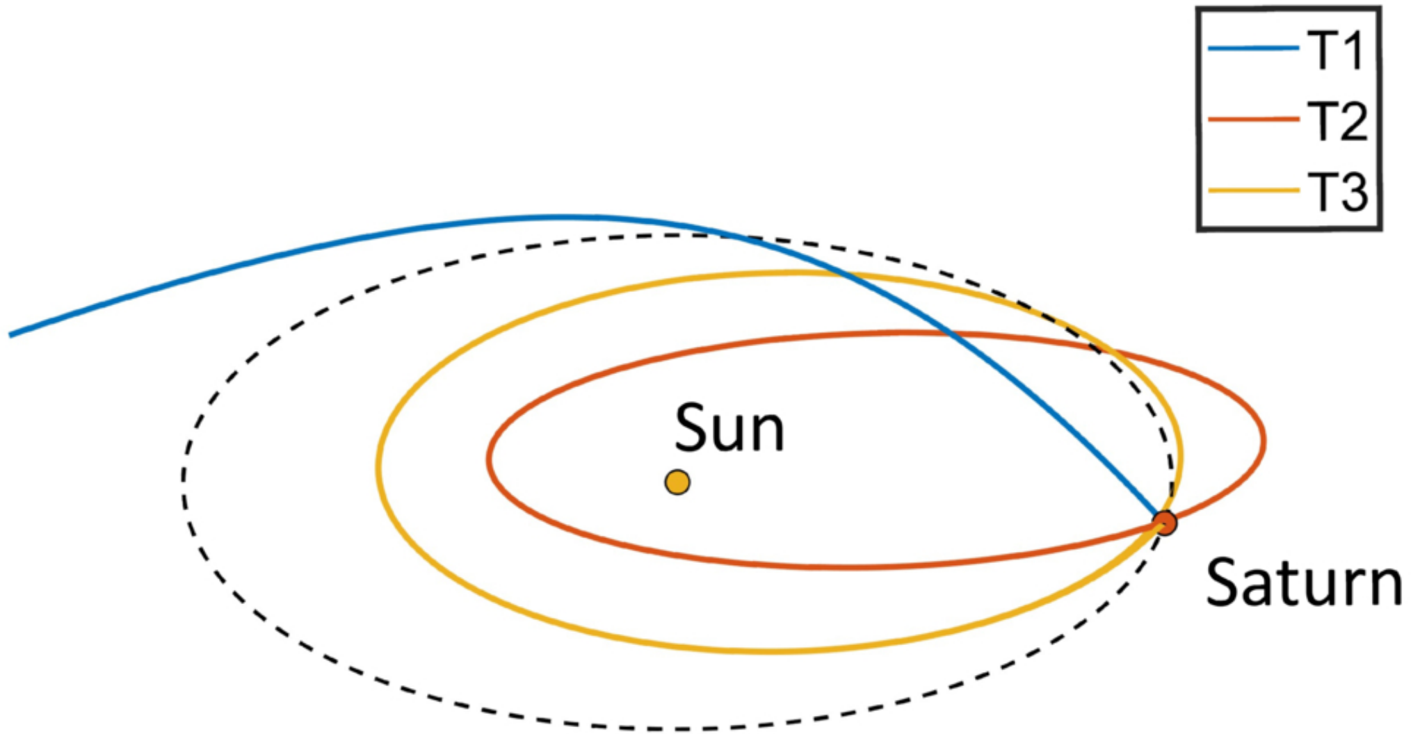
Figure 2. from Ian-Lin Lai et al 2026 Planet. Sci. J. 7 doi:10.3847/PSJ/aea848 https://dx.doi.org/10.3847/PSJ/aea848 © 2026. The Author(s). Published by the American Astronomical Society.
