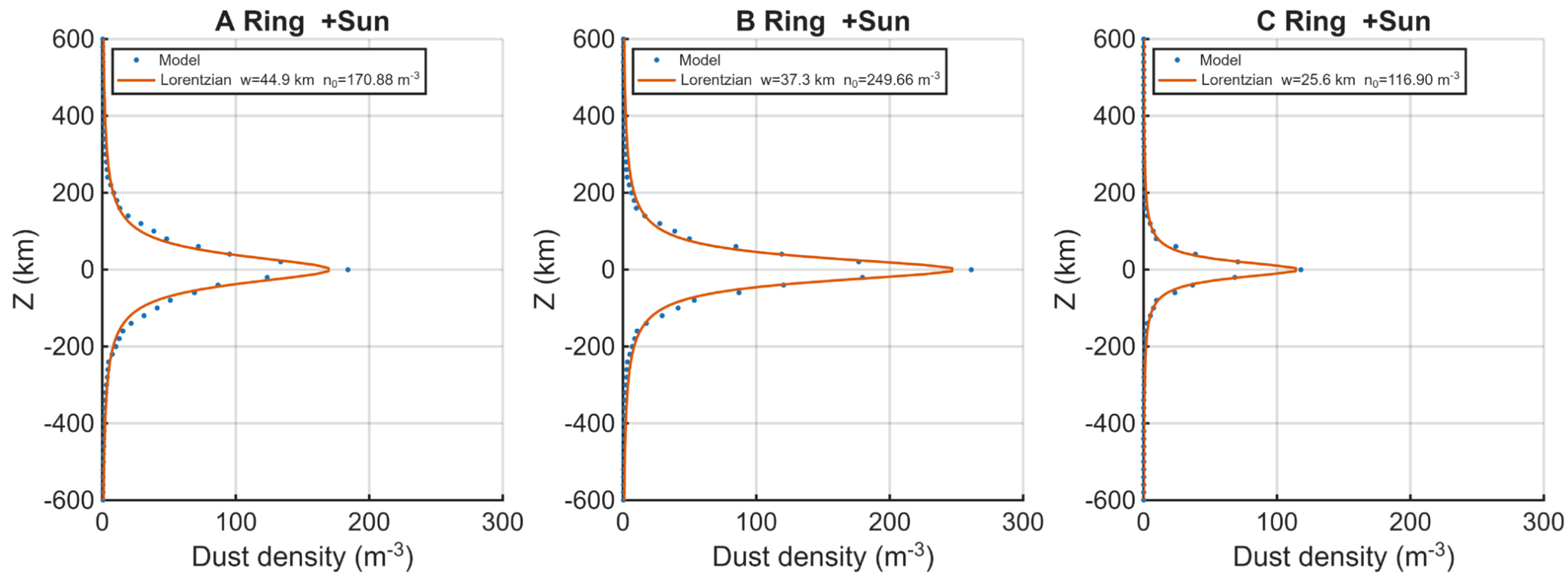
Figure 11. from Ian-Lin Lai et al 2026 Planet. Sci. J. 7 doi:10.3847/PSJ/aea848 https://dx.doi.org/10.3847/PSJ/aea848 © 2026. The Author(s). Published by the American Astronomical Society.
