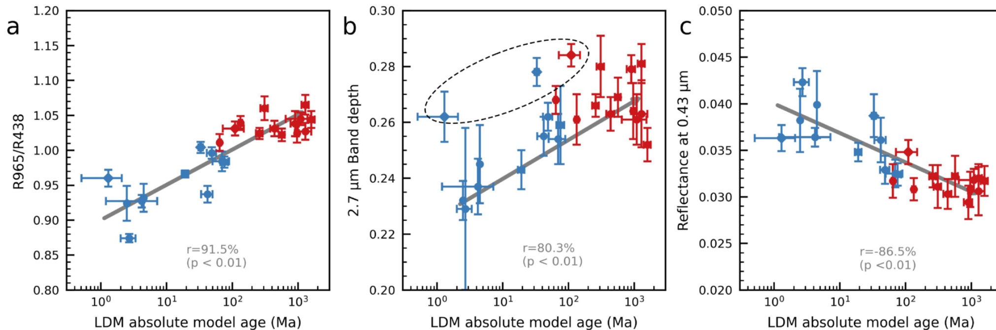
Figure 7. from Qing Zhang et al 2026 Planet. Sci. J. 7 doi:10.3847/PSJ/aea791 https://dx.doi.org/10.3847/PSJ/aea791 © 2026. The Author(s). Published by the American Astronomical Society.
