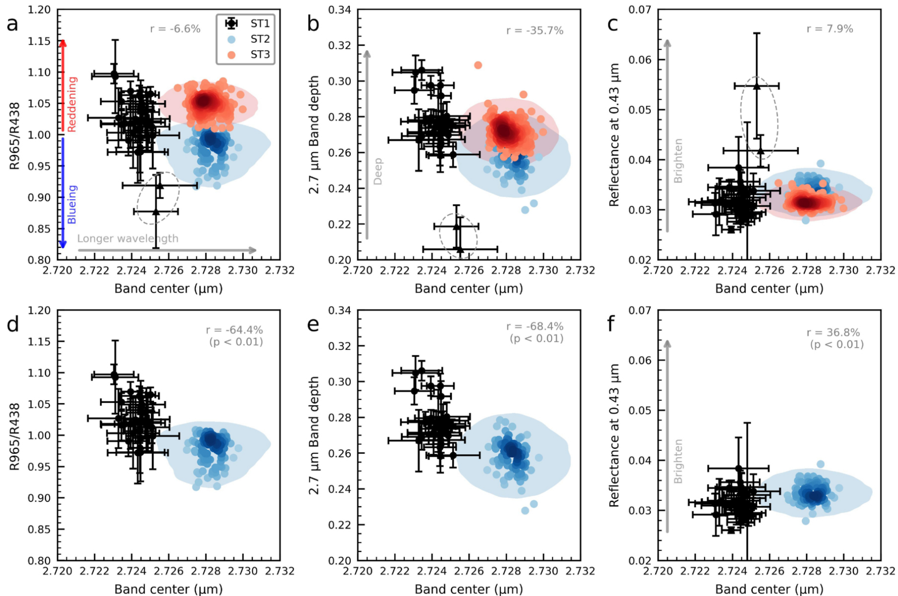
Figure 5. from Qing Zhang et al 2026 Planet. Sci. J. 7 doi:10.3847/PSJ/aea791 https://dx.doi.org/10.3847/PSJ/aea791 © 2026. The Author(s). Published by the American Astronomical Society.
