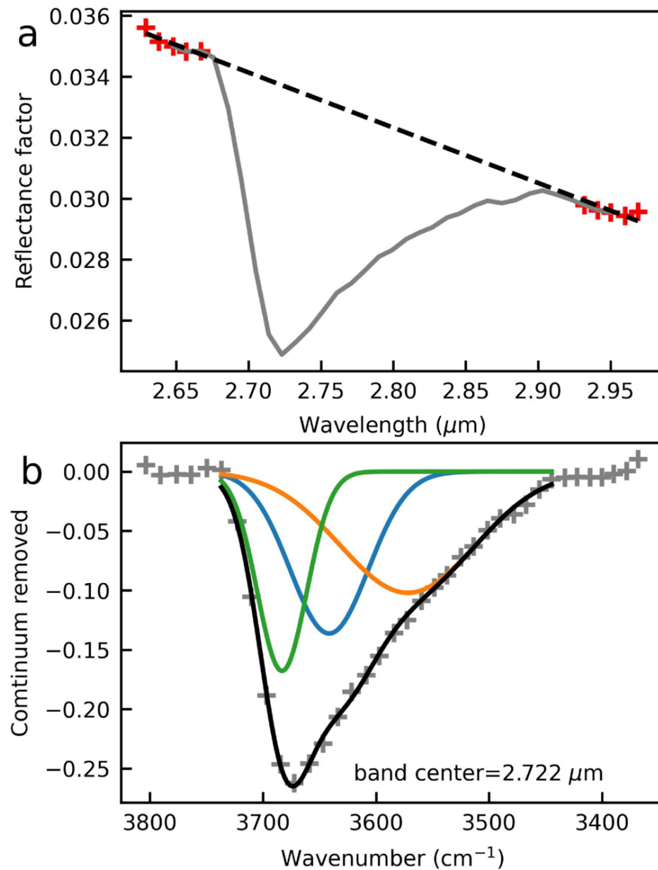
Figure 1. from Qing Zhang et al 2026 Planet. Sci. J. 7 doi:10.3847/PSJ/aea791 https://dx.doi.org/10.3847/PSJ/aea791 © 2026. The Author(s). Published by the American Astronomical Society.
