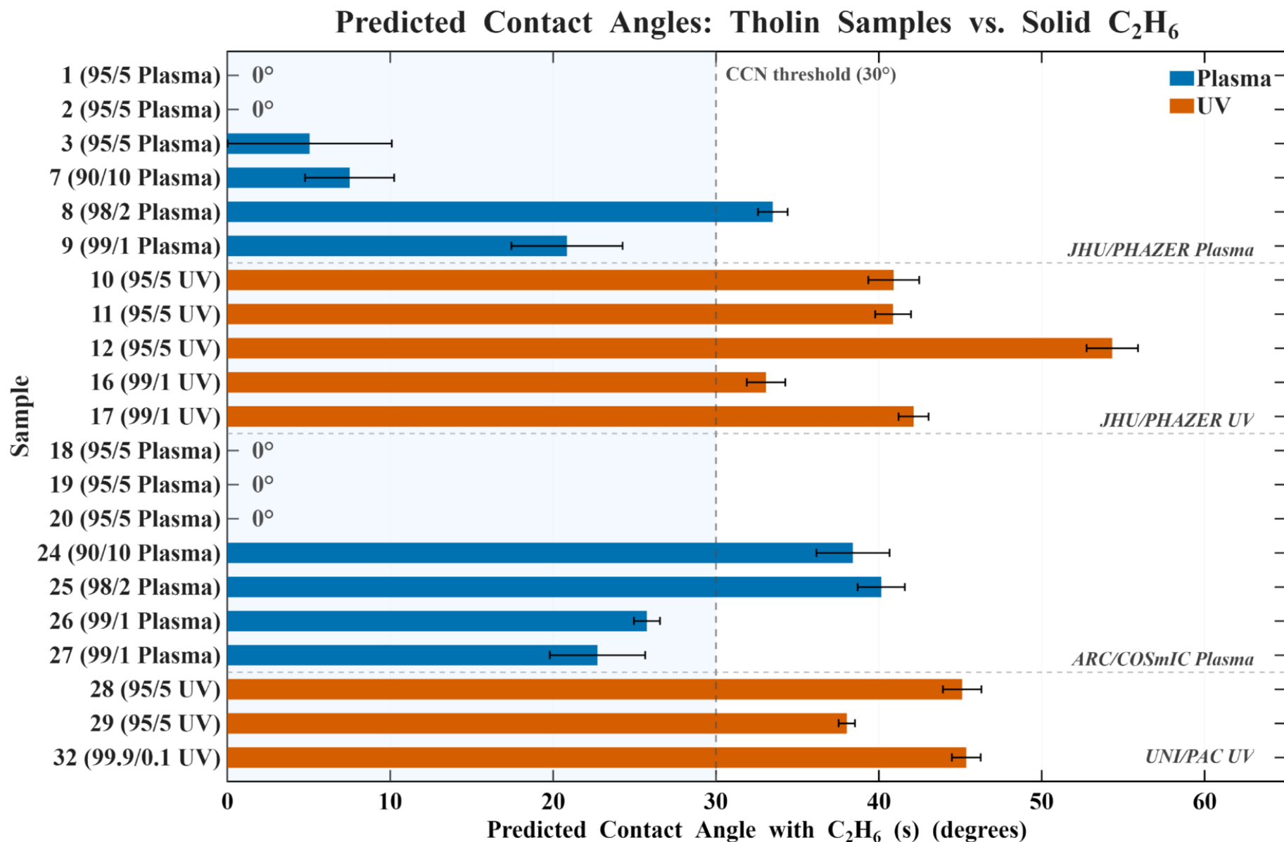
Figure 6. from Eric C. Austin et al 2026 Planet. Sci. J. 7 doi:10.3847/PSJ/aea60b https://dx.doi.org/10.3847/PSJ/aea60b © 2026. The Author(s). Published by the American Astronomical Society.
