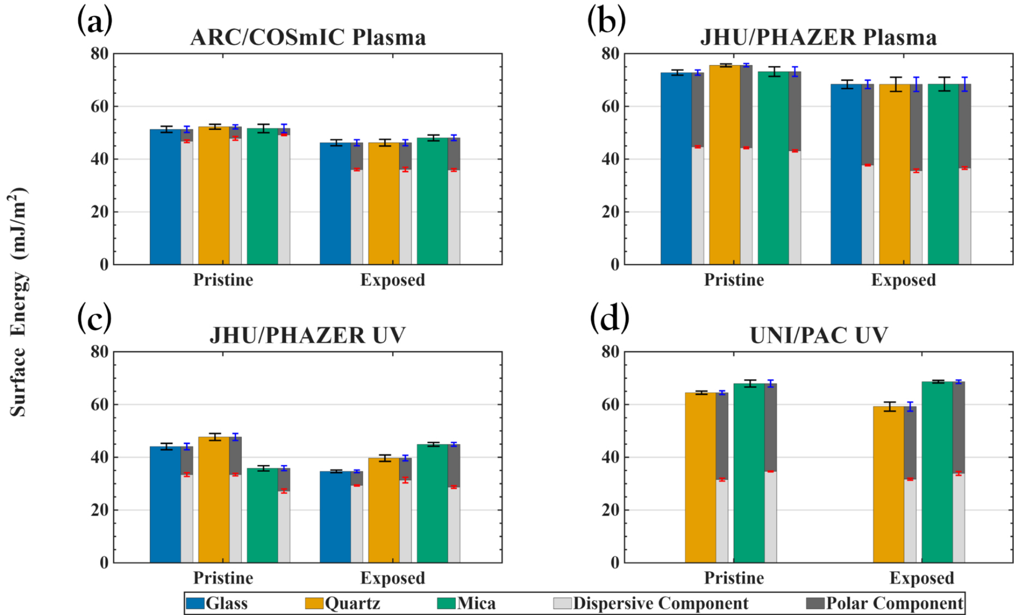
Figure 4. from Eric C. Austin et al 2026 Planet. Sci. J. 7 doi:10.3847/PSJ/aea60b https://dx.doi.org/10.3847/PSJ/aea60b © 2026. The Author(s). Published by the American Astronomical Society.
