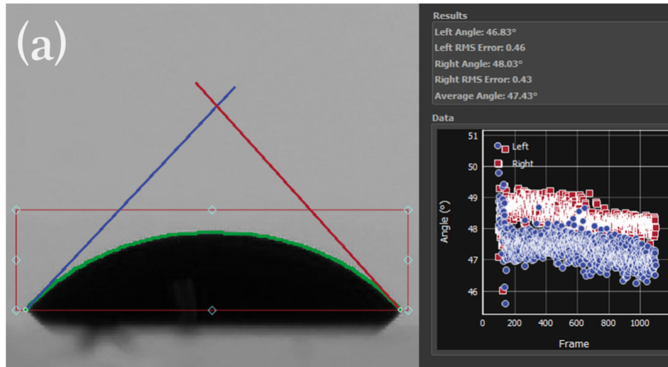
Figure 3. from Eric C. Austin et al 2026 Planet. Sci. J. 7 doi:10.3847/PSJ/aea60b https://dx.doi.org/10.3847/PSJ/aea60b © 2026. The Author(s). Published by the American Astronomical Society.
